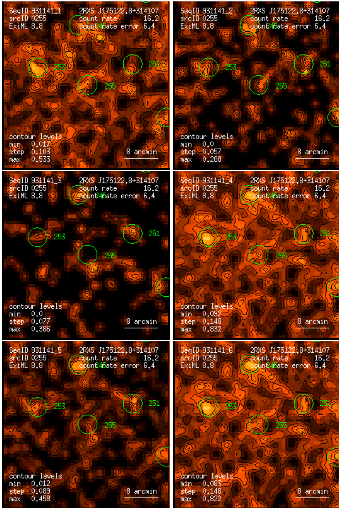
Figure 255: RASS 931141: detection 0255: band rate images, Gaussian filter: (1) PSPC channels 11 – 41, (2) 52 – 90, (3) 91 – 201, (4) 11 – 235, (5) 52 – 201, (6) 11 – 201. Broad band rates in counts/ks. Band rate contour levels in counts/ks/arcmin 2 .
