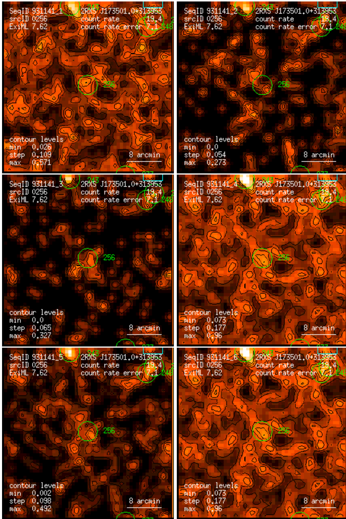
Figure 256: RASS 931141: detection 0256: band rate images, Gaussian filter: (1) PSPC channels 11 – 41, (2) 52 – 90, (3) 91 – 201, (4) 11 – 235, (5) 52 – 201, (6) 11 – 201. Broad band rates in counts/ks. Band rate contour levels in counts/ks/arcmin 2 .
