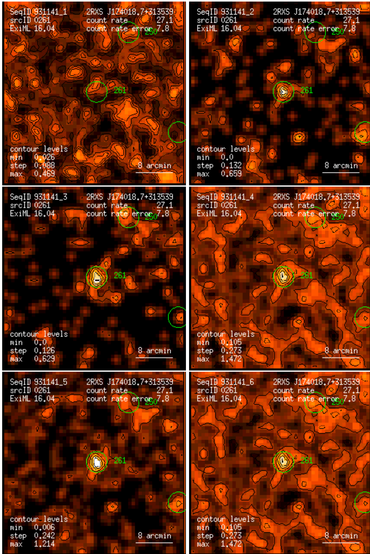
Figure 261: RASS 931141: detection 0261: band rate images, Gaussian filter: (1) PSPC channels 11 – 41, (2) 52 – 90, (3) 91 – 201, (4) 11 – 235, (5) 52 – 201, (6) 11 – 201. Broad band rates in counts/ks. Band rate contour levels in counts/ks/arcmin 2 .
