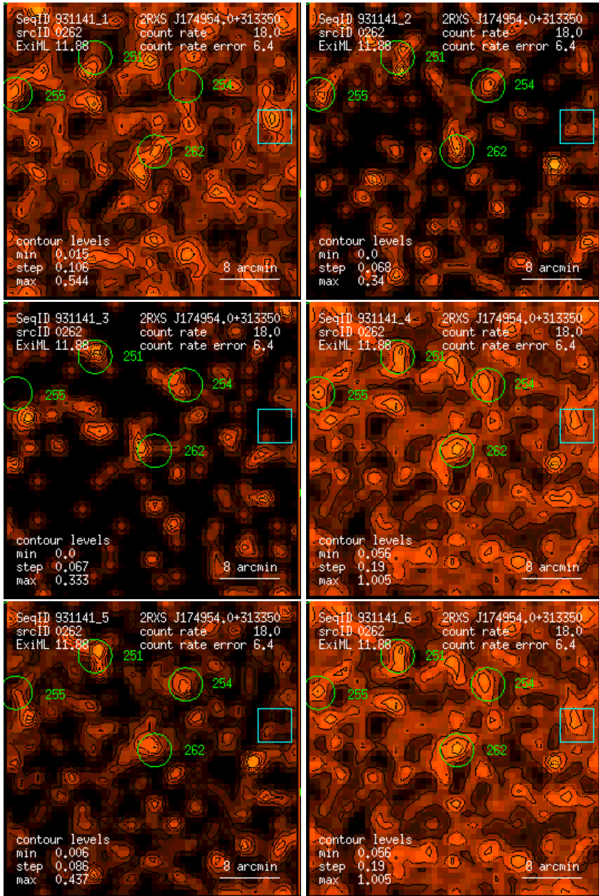
Figure 262: RASS 931141: detection 0262: band rate images, Gaussian filter: (1) PSPC channels 11 – 41, (2) 52 – 90, (3) 91 – 201, (4) 11 – 235, (5) 52 – 201, (6) 11 – 201. Broad band rates in counts/ks. Band rate contour levels in counts/ks/arcmin 2 .
