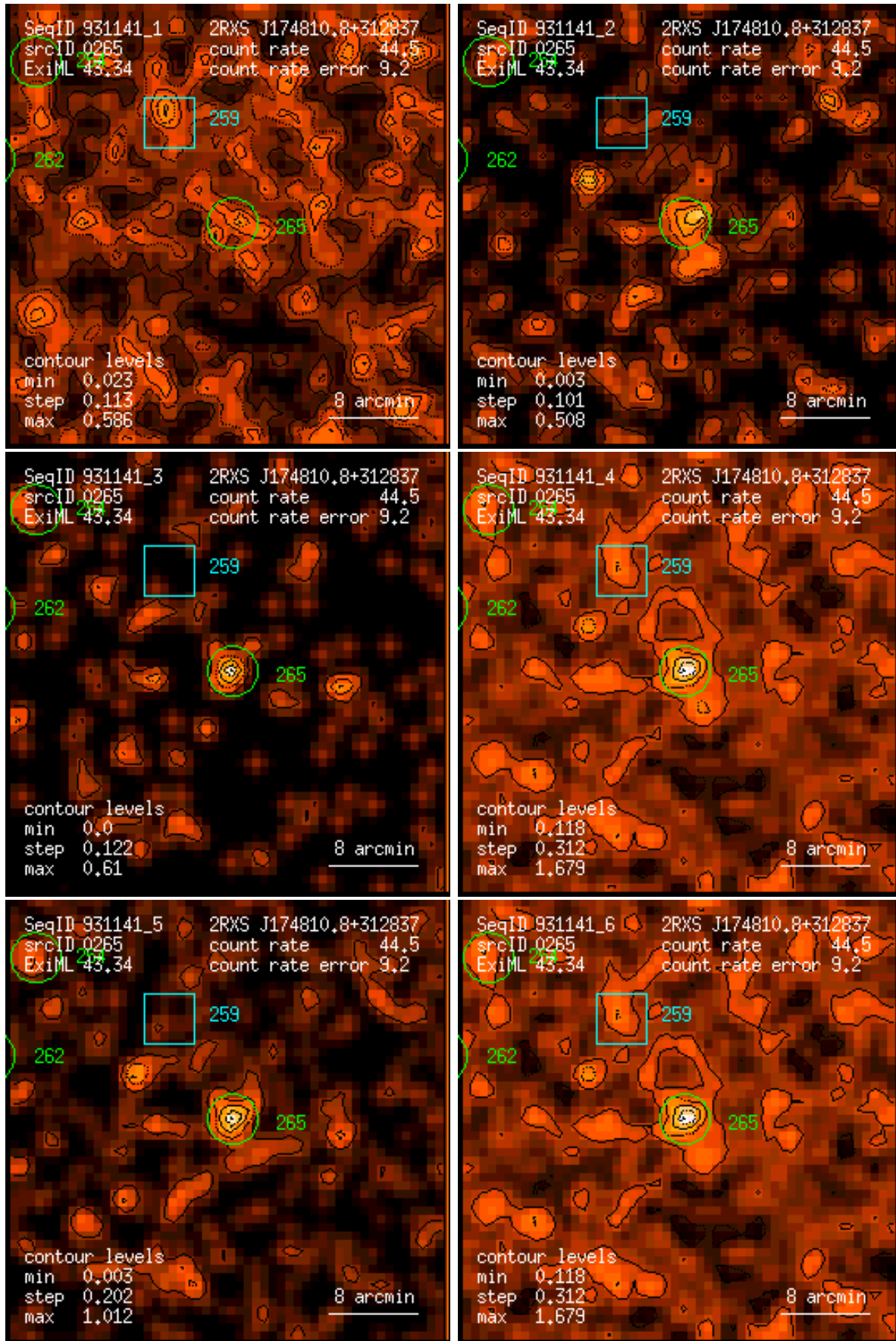
Figure 265: RASS 931141: detection 0265: band rate images, Gaussian filter: (1) PSPC channels 11 – 41, (2) 52 – 90, (3) 91 – 201, (4) 11 – 235, (5) 52 – 201, (6) 11 – 201. Broad band rates in counts/ks. Band rate contour levels in counts/ks/arcmin 2 .
