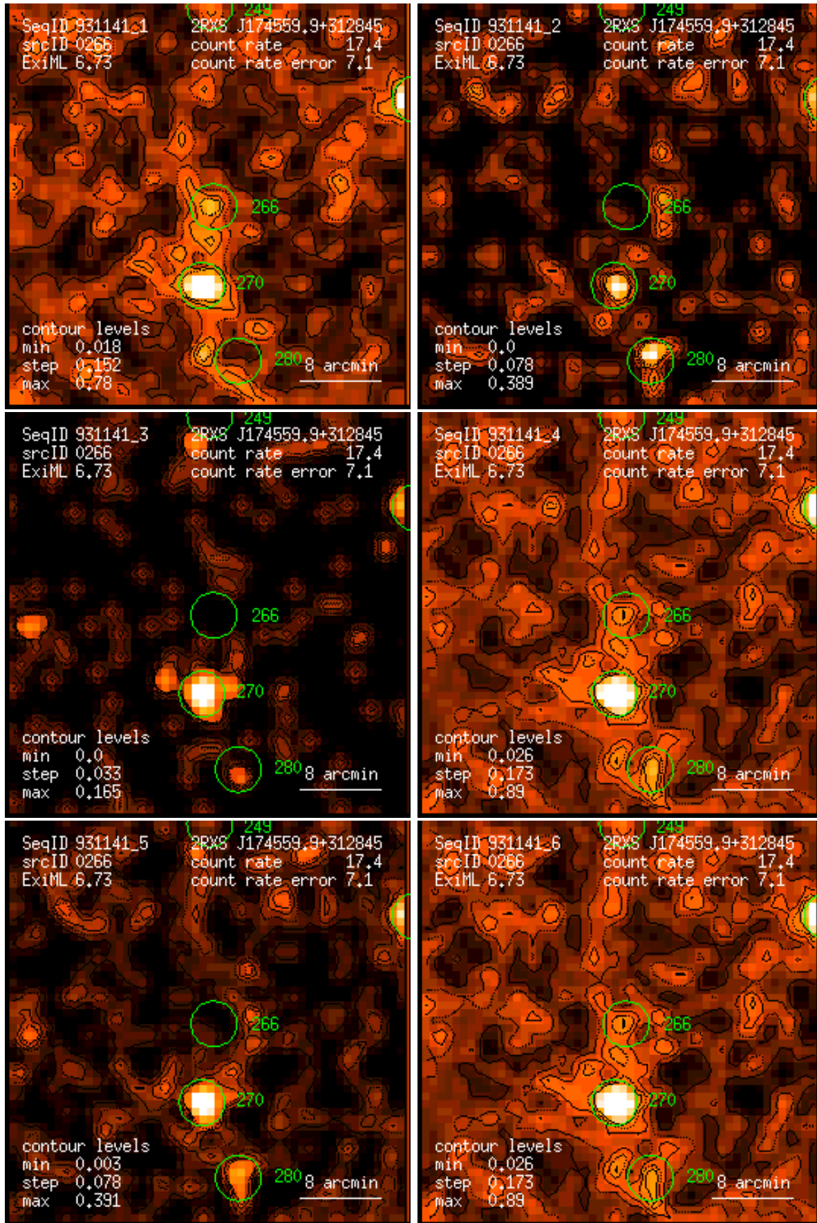
Figure 266: RASS 931141: detection 0266: band rate images, Gaussian filter: (1) PSPC channels 11 – 41, (2) 52 – 90, (3) 91 – 201, (4) 11 – 235, (5) 52 – 201, (6) 11 – 201. Broad band rates in counts/ks. Band rate contour levels in counts/ks/arcmin 2 .
