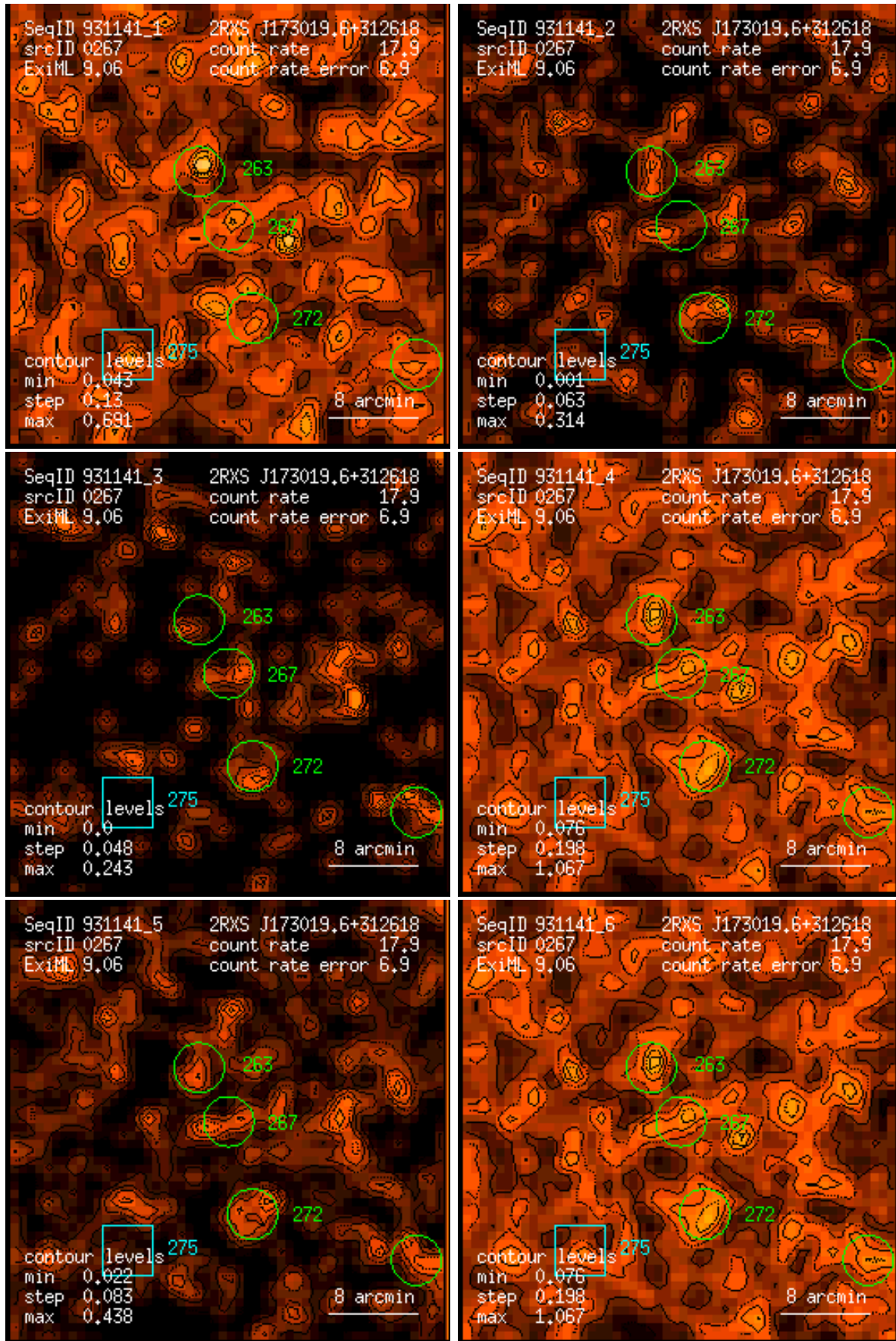
Figure 267: RASS 931141: detection 0267: band rate images, Gaussian filter: (1) PSPC channels 11 – 41, (2) 52 – 90, (3) 91 – 201, (4) 11 – 235, (5) 52 – 201, (6) 11 – 201. Broad band rates in counts/ks. Band rate contour levels in counts/ks/arcmin 2 .
