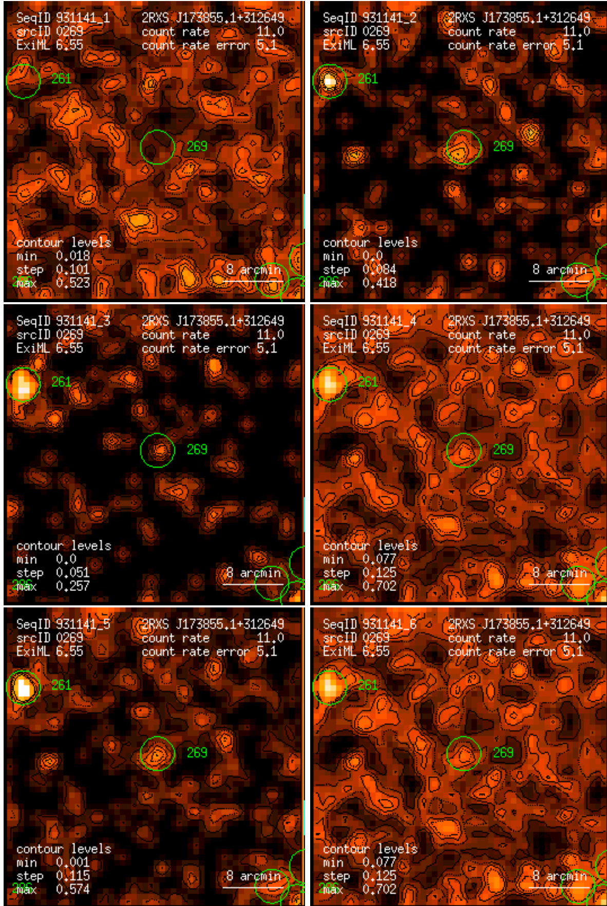
Figure 269: RASS 931141: detection 0269: band rate images, Gaussian filter: (1) PSPC channels 11 – 41, (2) 52 – 90, (3) 91 – 201, (4) 11 – 235, (5) 52 – 201, (6) 11 – 201. Broad band rates in counts/ks. Band rate contour levels in counts/ks/arcmin 2 .
