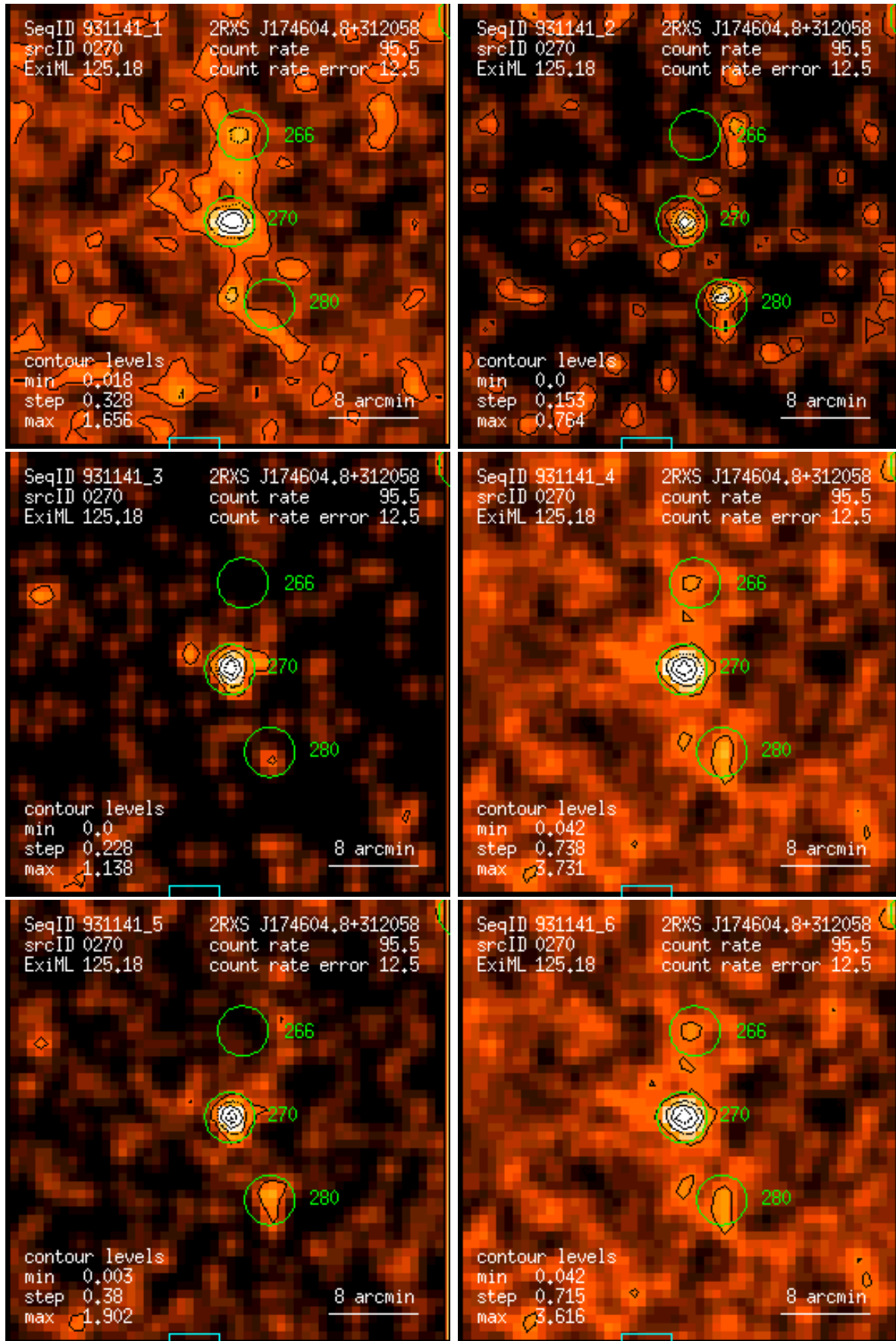
Figure 270: RASS 931141: detection 0270: band rate images, Gaussian filter: (1) PSPC channels 11 – 41, (2) 52 – 90, (3) 91 – 201, (4) 11 – 235, (5) 52 – 201, (6) 11 – 201. Broad band rates in counts/ks. Band rate contour levels in counts/ks/arcmin 2 .
