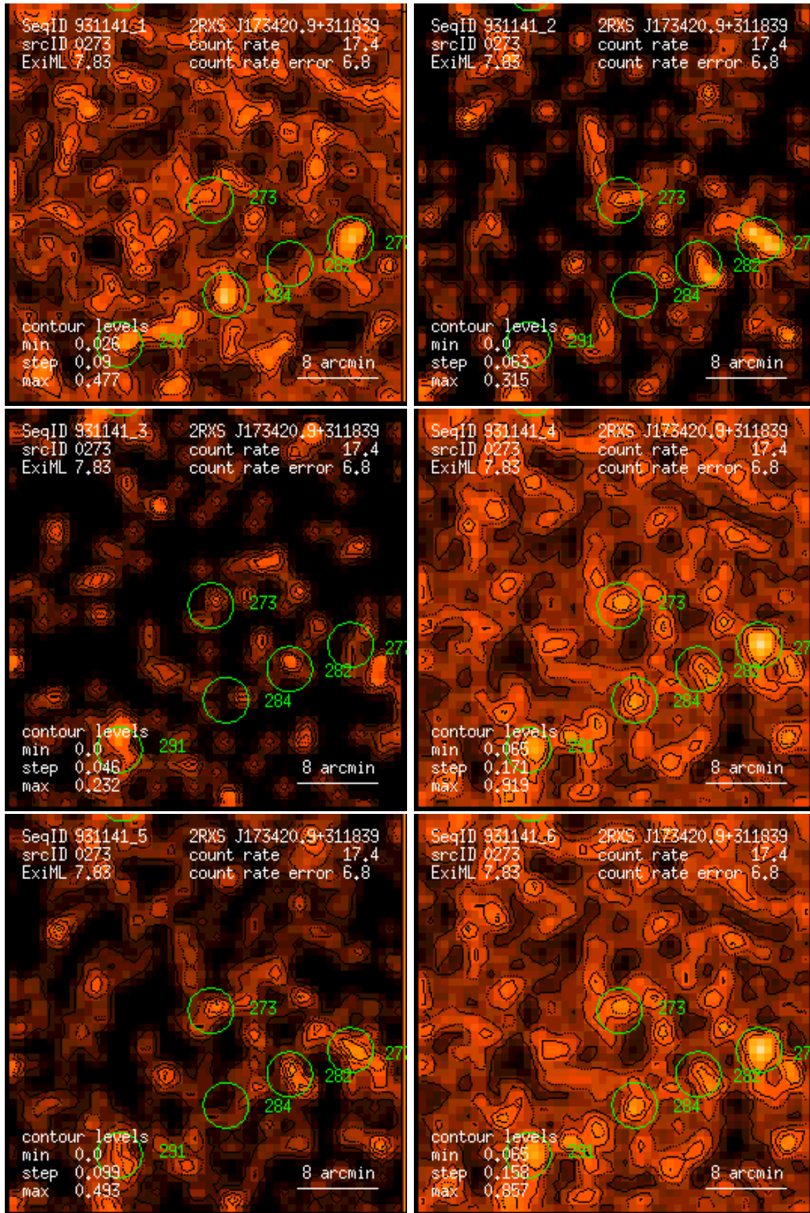
Figure 273: RASS 931141: detection 0273: band rate images, Gaussian filter: (1) PSPC channels 11 – 41, (2) 52 – 90, (3) 91 – 201, (4) 11 – 235, (5) 52 – 201, (6) 11 – 201. Broad band rates in counts/ks. Band rate contour levels in counts/ks/arcmin 2 .
