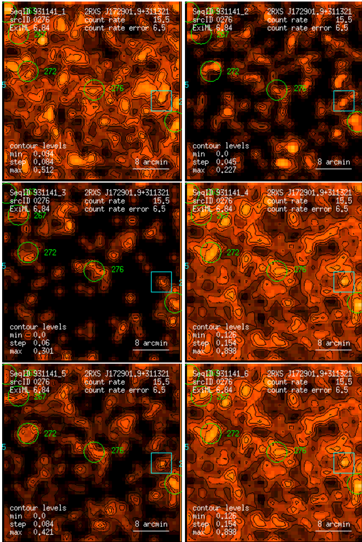
Figure 276: RASS 931141: detection 0276: band rate images, Gaussian filter: (1) PSPC channels 11 – 41, (2) 52 – 90, (3) 91 – 201, (4) 11 – 235, (5) 52 – 201, (6) 11 – 201. Broad band rates in counts/ks. Band rate contour levels in counts/ks/arcmin 2 .
