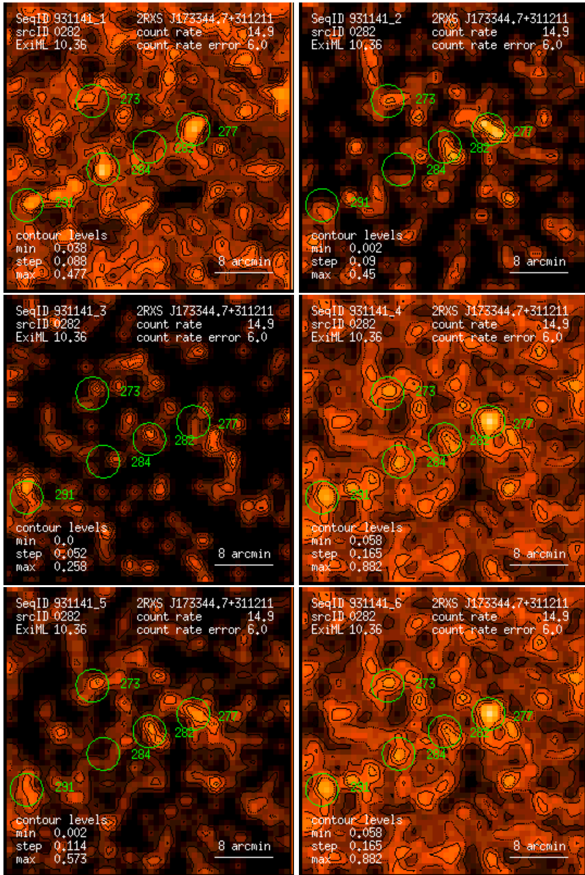
Figure 282: RASS 931141: detection 0282: band rate images, Gaussian filter: (1) PSPC channels 11 – 41, (2) 52 – 90, (3) 91 – 201, (4) 11 – 235, (5) 52 – 201, (6) 11 – 201. Broad band rates in counts/ks. Band rate contour levels in counts/ks/arcmin 2 .
