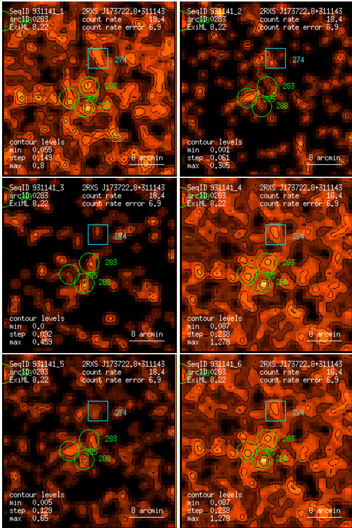
Figure 283: RASS 931141: detection 0283: band rate images, Gaussian filter: (1) PSPC channels 11 – 41, (2) 52 – 90, (3) 91 – 201, (4) 11 – 235, (5) 52 – 201, (6) 11 – 201. Broad band rates in counts/ks. Band rate contour levels in counts/ks/arcmin 2 .
