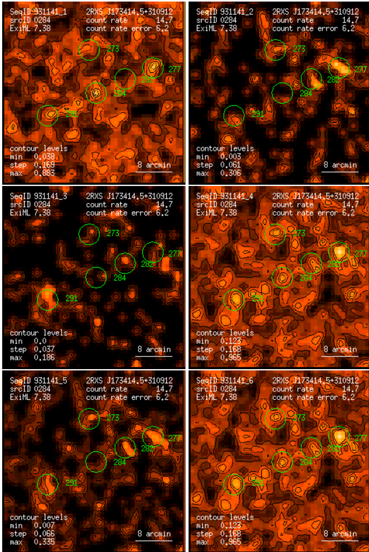
Figure 284: RASS 931141: detection 0284: band rate images, Gaussian filter: (1) PSPC channels 11 – 41, (2) 52 – 90, (3) 91 – 201, (4) 11 – 235, (5) 52 – 201, (6) 11 – 201. Broad band rates in counts/ks. Band rate contour levels in counts/ks/arcmin 2 .
