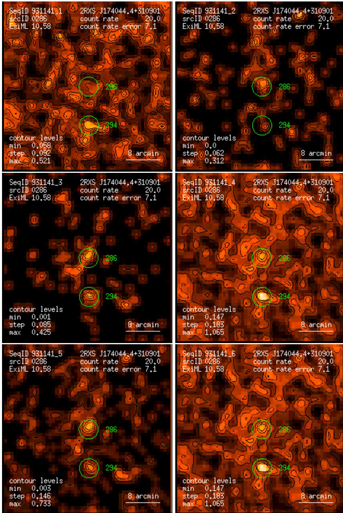
Figure 286: RASS 931141: detection 0286: band rate images, Gaussian filter: (1) PSPC channels 11 – 41, (2) 52 – 90, (3) 91 – 201, (4) 11 – 235, (5) 52 – 201, (6) 11 – 201. Broad band rates in counts/ks. Band rate contour levels in counts/ks/arcmin 2 .
