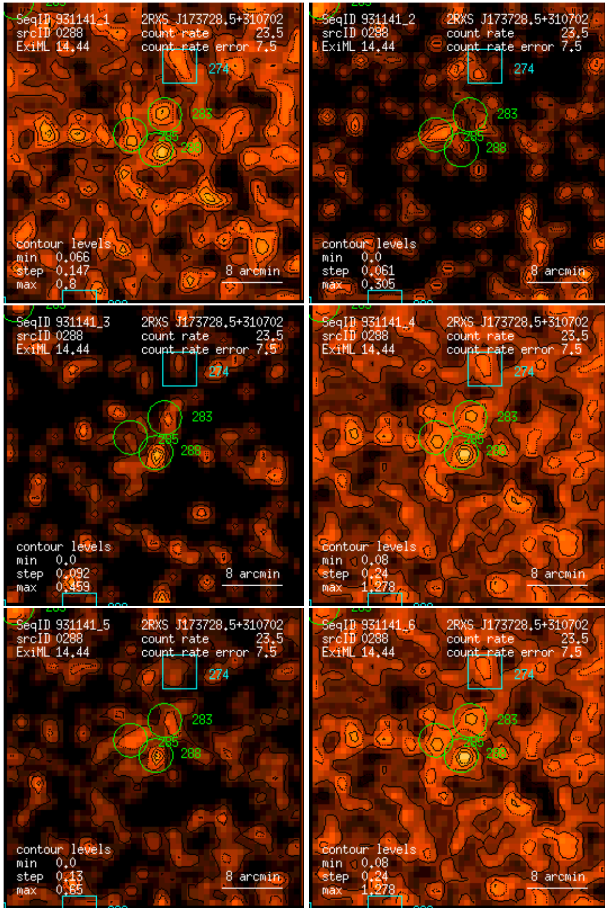
Figure 288: RASS 931141: detection 0288: band rate images, Gaussian filter: (1) PSPC channels 11 – 41, (2) 52 – 90, (3) 91 – 201, (4) 11 – 235, (5) 52 – 201, (6) 11 – 201. Broad band rates in counts/ks. Band rate contour levels in counts/ks/arcmin 2 .
