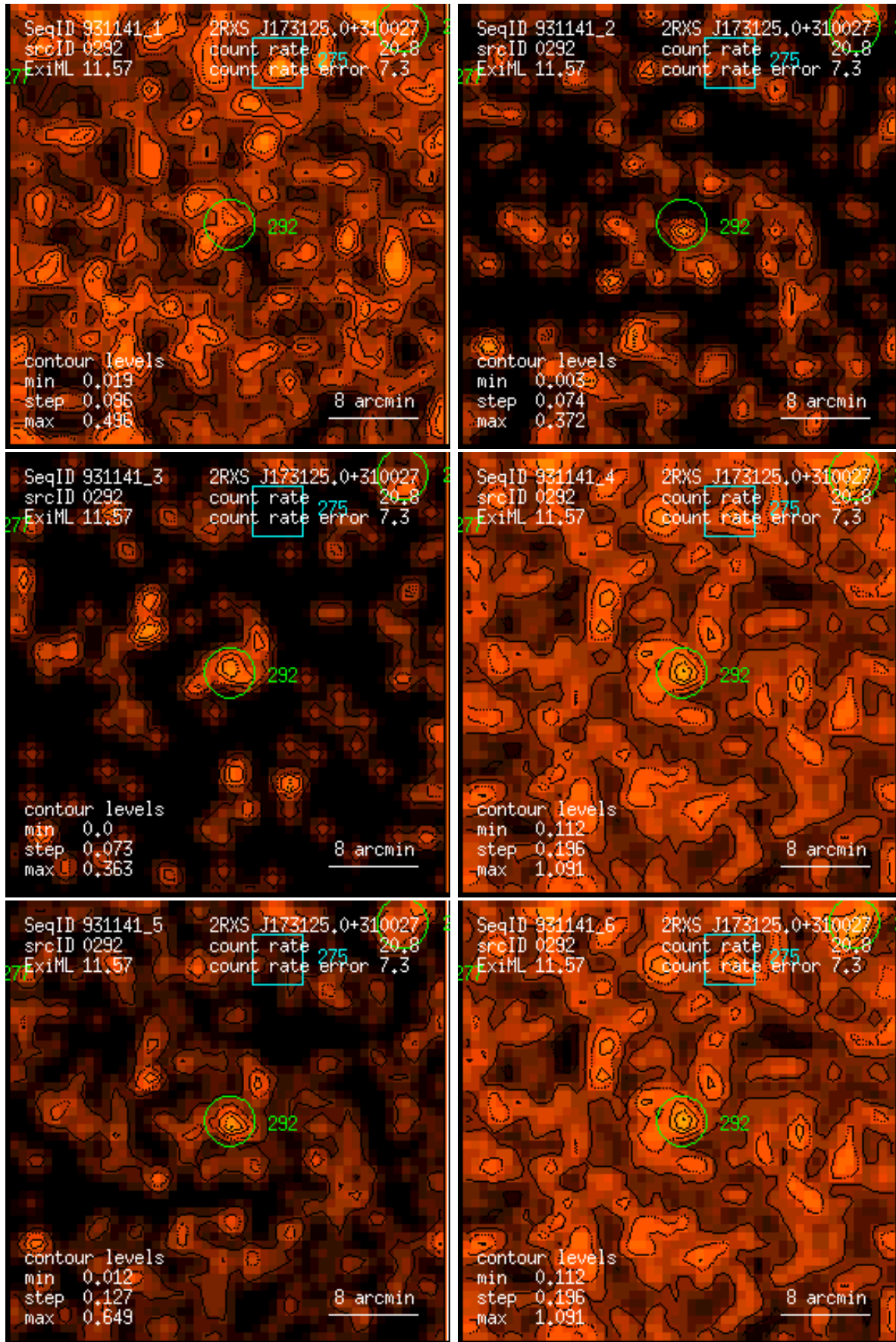
Figure 292: RASS 931141: detection 0292: band rate images, Gaussian filter: (1) PSPC channels 11 – 41, (2) 52 – 90, (3) 91 – 201, (4) 11 – 235, (5) 52 – 201, (6) 11 – 201. Broad band rates in counts/ks. Band rate contour levels in counts/ks/arcmin 2 .
