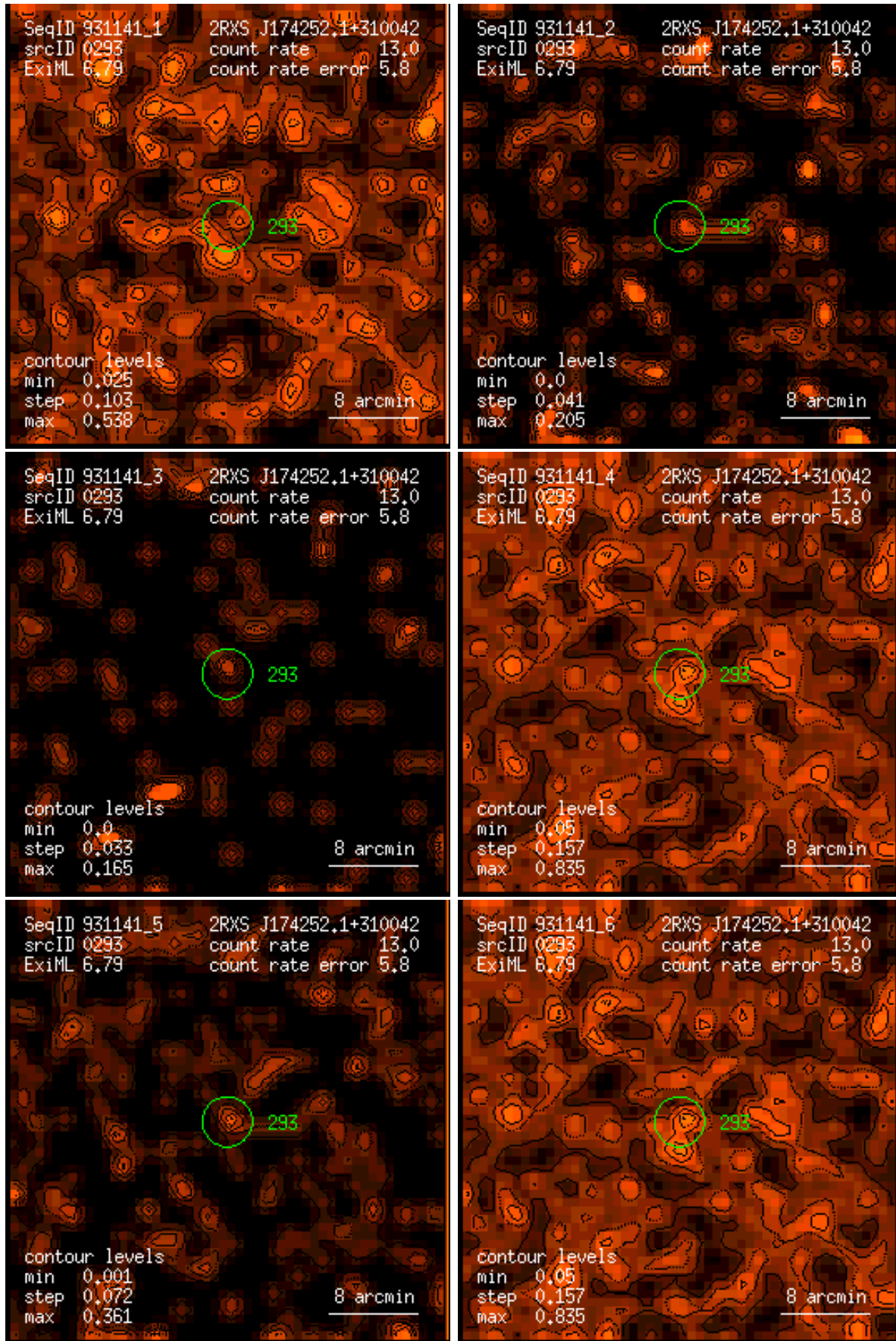
Figure 293: RASS 931141: detection 0293: band rate images, Gaussian filter: (1) PSPC channels 11 – 41, (2) 52 – 90, (3) 91 – 201, (4) 11 – 235, (5) 52 – 201, (6) 11 – 201. Broad band rates in counts/ks. Band rate contour levels in counts/ks/arcmin 2 .
