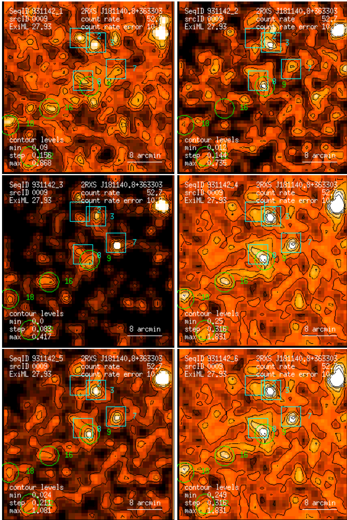
Figure 9: RASS 931142: detection 0009: band rate images, Gaussian filter: (1) PSPC channels 11 – 41, (2) 52 – 90, (3) 91 – 201, (4) 11 – 235, (5) 52 – 201, (6) 11 – 201. Broad band rates in counts/ks. Band rate contour levels in counts/ks/arcmin 2 .
