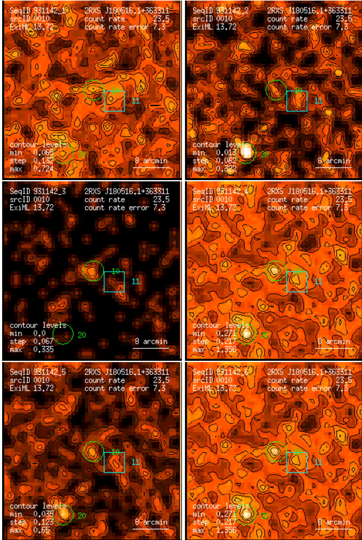
Figure 10: RASS 931142: detection 0010: band rate images, Gaussian filter: (1) PSPC channels 11 – 41, (2) 52 – 90, (3) 91 – 201, (4) 11 – 235, (5) 52 – 201, (6) 11 – 201. Broad band rates in counts/ks. Band rate contour levels in counts/ks/arcmin 2 .
