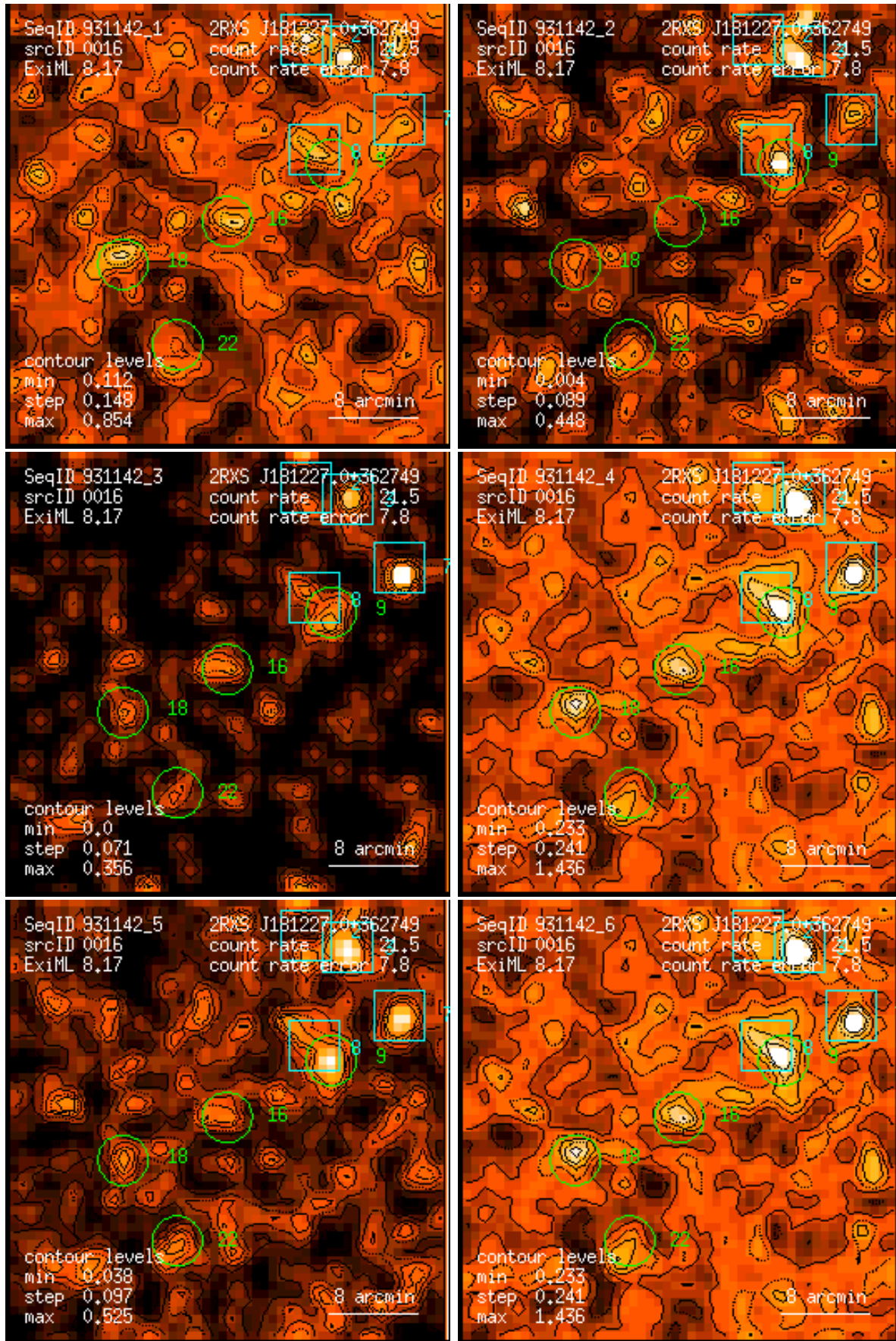
Figure 16: RASS 931142: detection 0016: band rate images, Gaussian filter: (1) PSPC channels 11 – 41, (2) 52 – 90, (3) 91 – 201, (4) 11 – 235, (5) 52 – 201, (6) 11 – 201. Broad band rates in counts/ks. Band rate contour levels in counts/ks/arcmin 2 .
