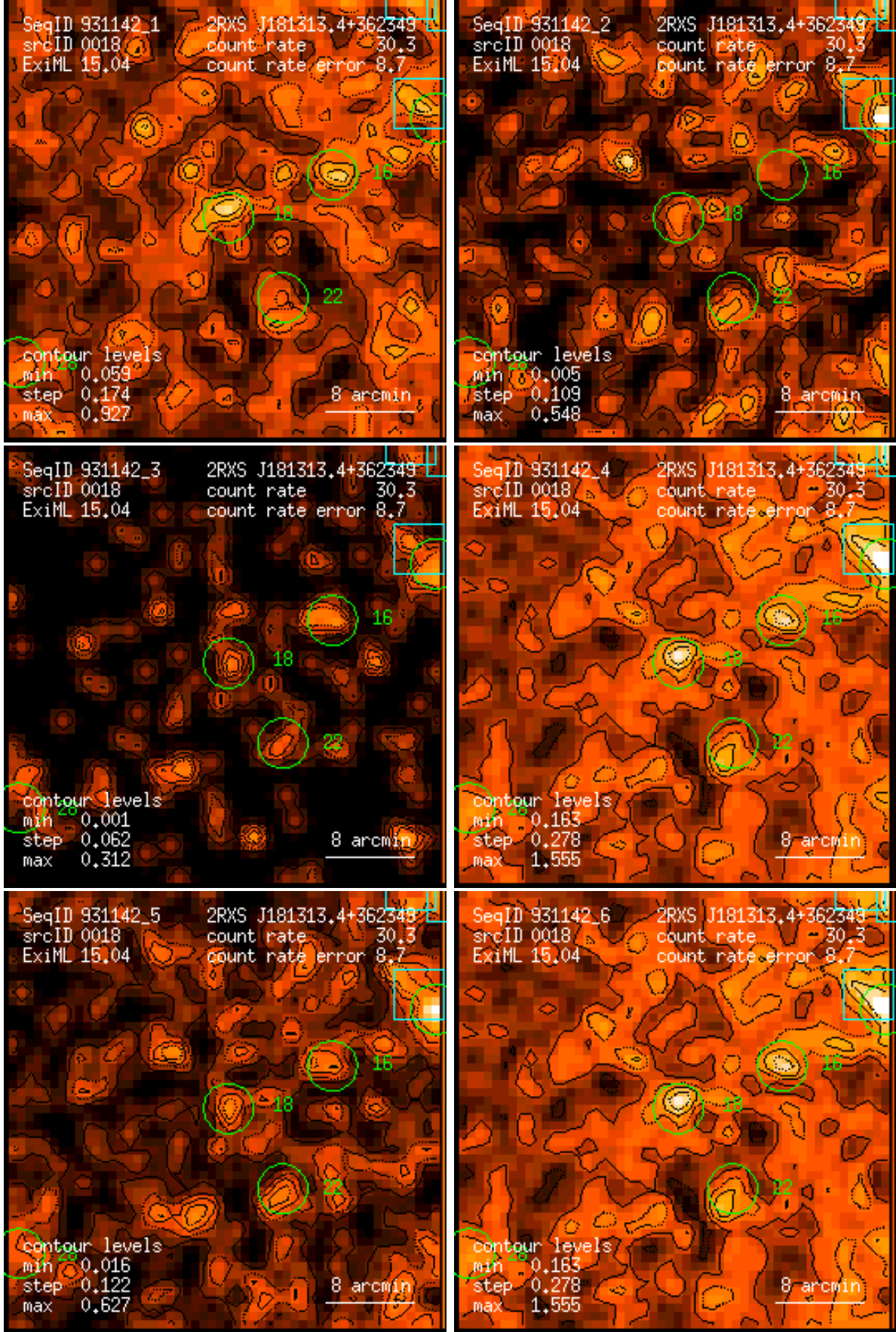
Figure 18: RASS 931142: detection 0018: band rate images, Gaussian filter: (1) PSPC channels 11 – 41, (2) 52 – 90, (3) 91 – 201, (4) 11 – 235, (5) 52 – 201, (6) 11 – 201. Broad band rates in counts/ks. Band rate contour levels in counts/ks/arcmin 2 .
