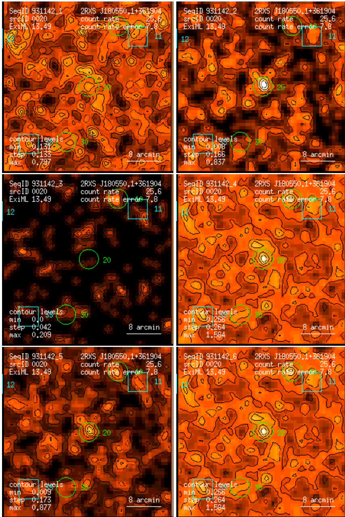
Figure 20: RASS 931142: detection 0020: band rate images, Gaussian filter: (1) PSPC channels 11 – 41, (2) 52 – 90, (3) 91 – 201, (4) 11 – 235, (5) 52 – 201, (6) 11 – 201. Broad band rates in counts/ks. Band rate contour levels in counts/ks/arcmin 2 .
