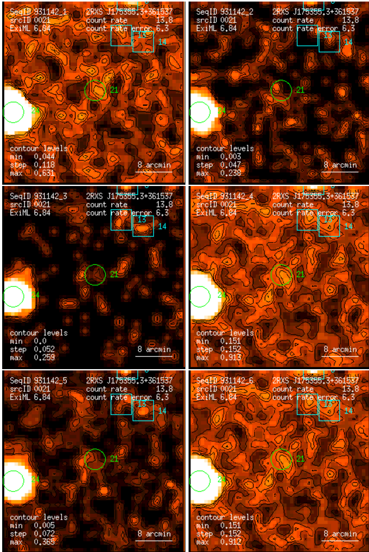
Figure 21: RASS 931142: detection 0021: band rate images, Gaussian filter: (1) PSPC channels 11 – 41, (2) 52 – 90, (3) 91 – 201, (4) 11 – 235, (5) 52 – 201, (6) 11 – 201. Broad band rates in counts/ks. Band rate contour levels in counts/ks/arcmin 2 .
