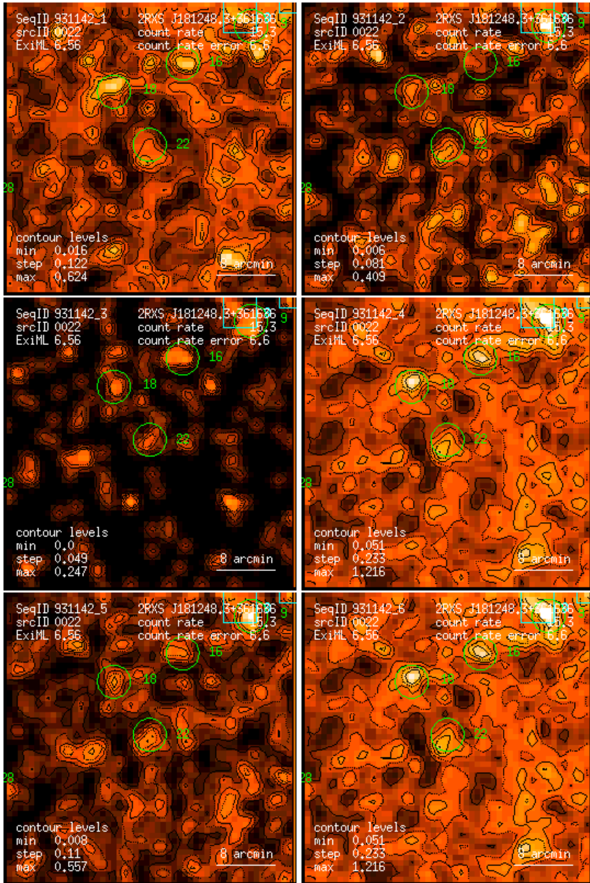
Figure 22: RASS 931142: detection 0022: band rate images, Gaussian filter: (1) PSPC channels 11 – 41, (2) 52 – 90, (3) 91 – 201, (4) 11 – 235, (5) 52 – 201, (6) 11 – 201. Broad band rates in counts/ks. Band rate contour levels in counts/ks/arcmin 2 .
