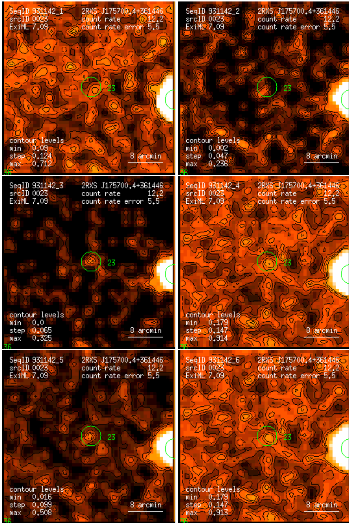
Figure 23: RASS 931142: detection 0023: band rate images, Gaussian filter: (1) PSPC channels 11 – 41, (2) 52 – 90, (3) 91 – 201, (4) 11 – 235, (5) 52 – 201, (6) 11 – 201. Broad band rates in counts/ks. Band rate contour levels in counts/ks/arcmin 2 .
