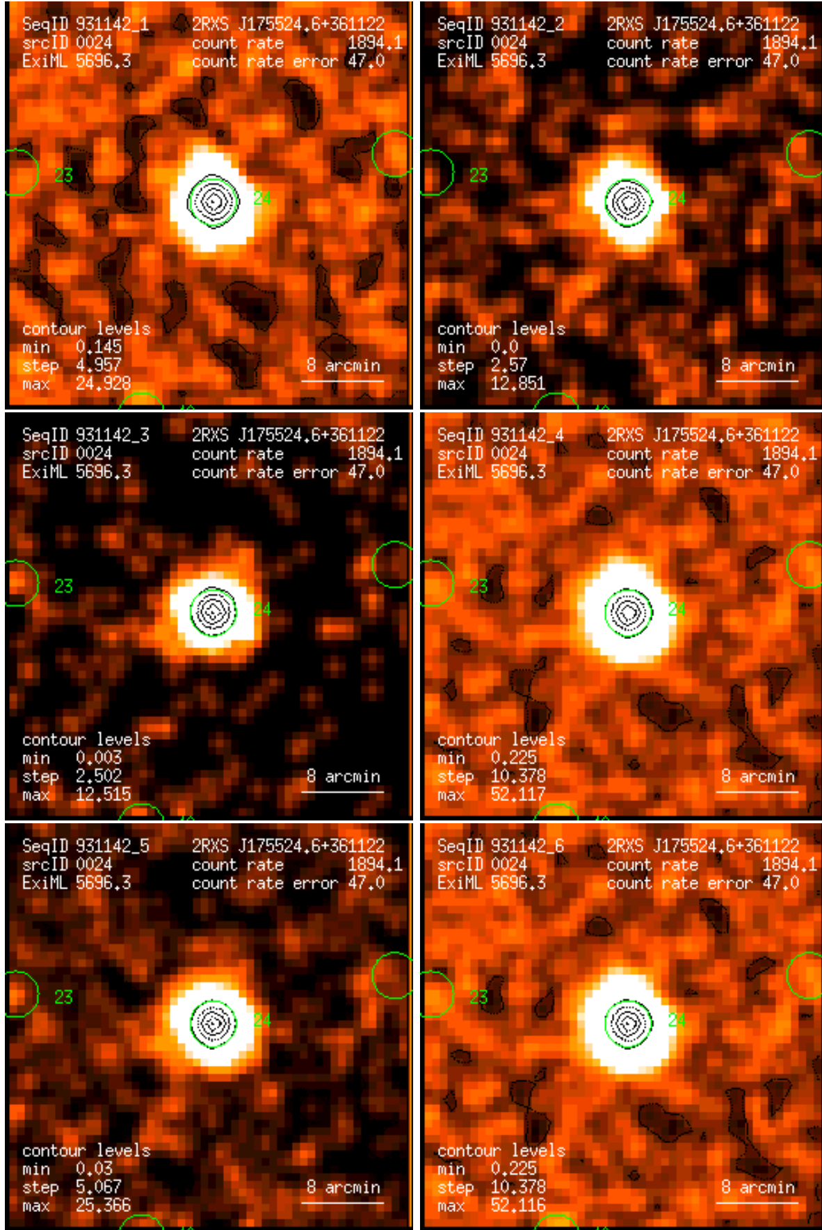
Figure 24: RASS 931142: detection 0024: band rate images, Gaussian filter: (1) PSPC channels 11 – 41, (2) 52 – 90, (3) 91 – 201, (4) 11 – 235, (5) 52 – 201, (6) 11 – 201. Broad band rates in counts/ks. Band rate contour levels in counts/ks/arcmin 2 .
