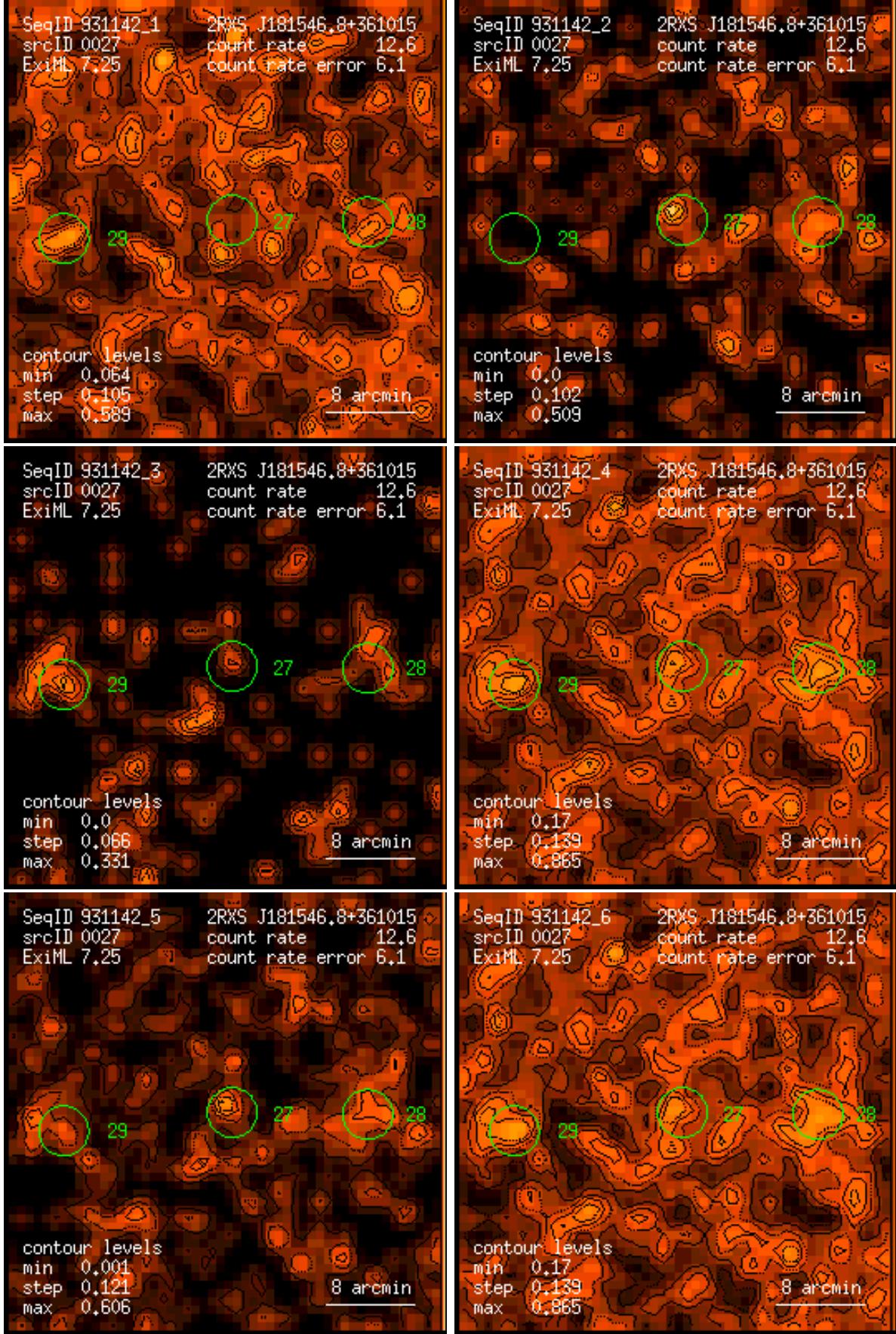
Figure 27: RASS 931142: detection 0027: band rate images, Gaussian filter: (1) PSPC channels 11 – 41, (2) 52 – 90, (3) 91 – 201, (4) 11 – 235, (5) 52 – 201, (6) 11 – 201. Broad band rates in counts/ks. Band rate contour levels in counts/ks/arcmin 2 .
