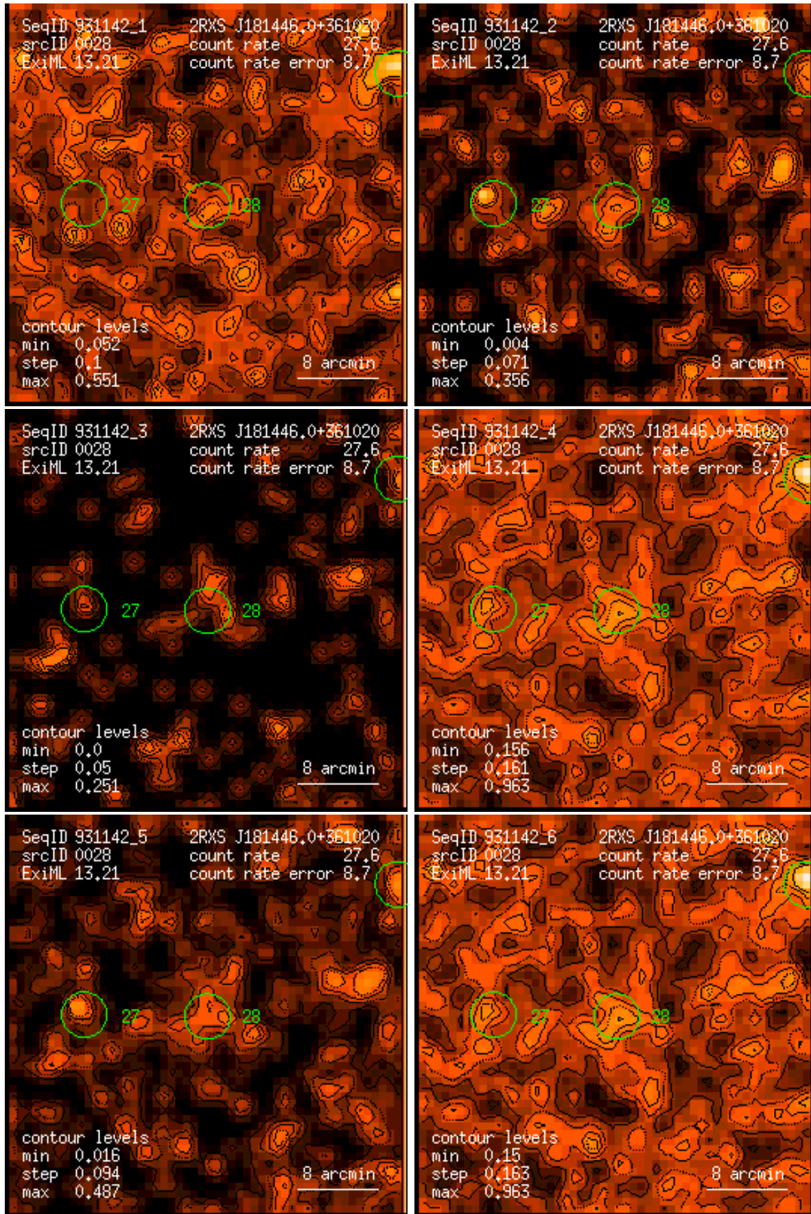
Figure 28: RASS 931142: detection 0028: band rate images, Gaussian filter: (1) PSPC channels 11 – 41, (2) 52 – 90, (3) 91 – 201, (4) 11 – 235, (5) 52 – 201, (6) 11 – 201. Broad band rates in counts/ks. Band rate contour levels in counts/ks/arcmin 2 .
