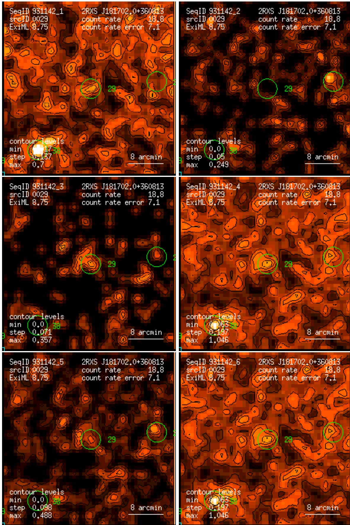
Figure 29: RASS 931142: detection 0029: band rate images, Gaussian filter: (1) PSPC channels 11 – 41, (2) 52 – 90, (3) 91 – 201, (4) 11 – 235, (5) 52 – 201, (6) 11 – 201. Broad band rates in counts/ks. Band rate contour levels in counts/ks/arcmin 2 .
