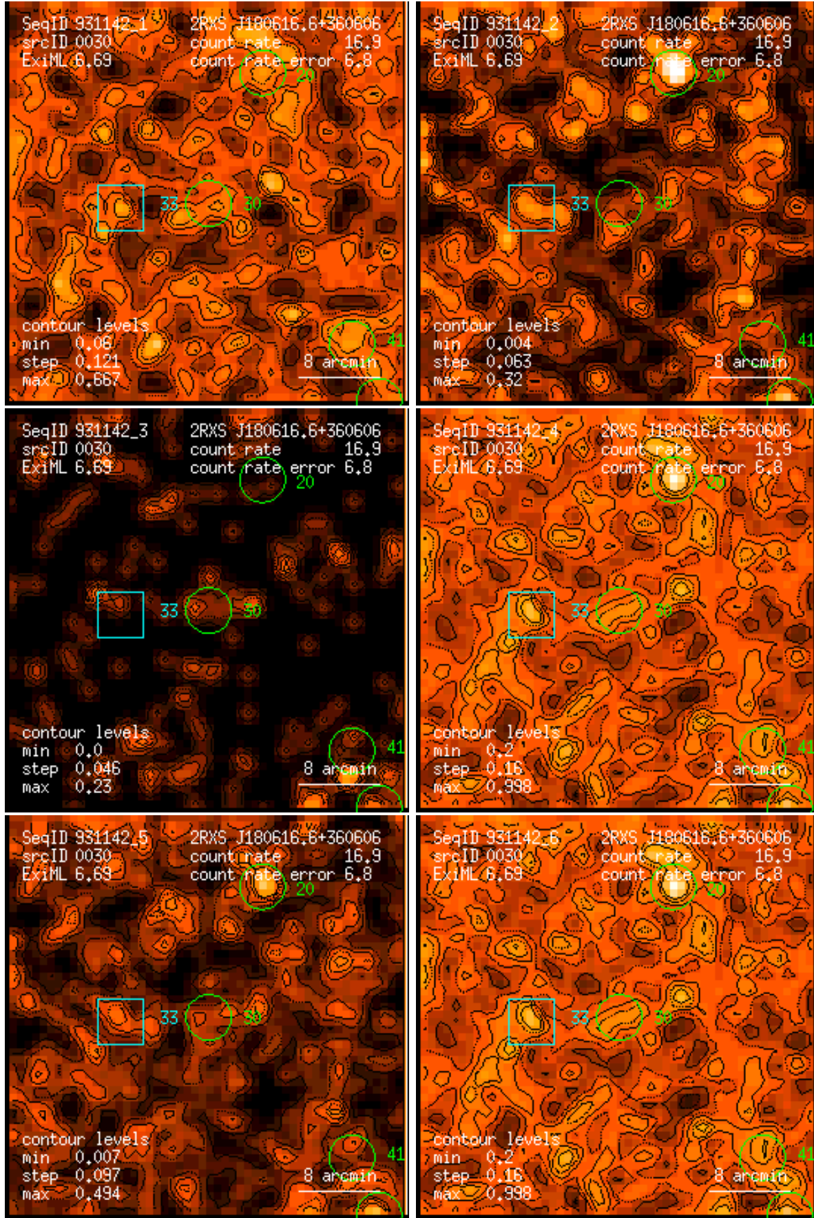
Figure 30: RASS 931142: detection 0030: band rate images, Gaussian filter: (1) PSPC channels 11 – 41, (2) 52 – 90, (3) 91 – 201, (4) 11 – 235, (5) 52 – 201, (6) 11 – 201. Broad band rates in counts/ks. Band rate contour levels in counts/ks/arcmin 2 .
