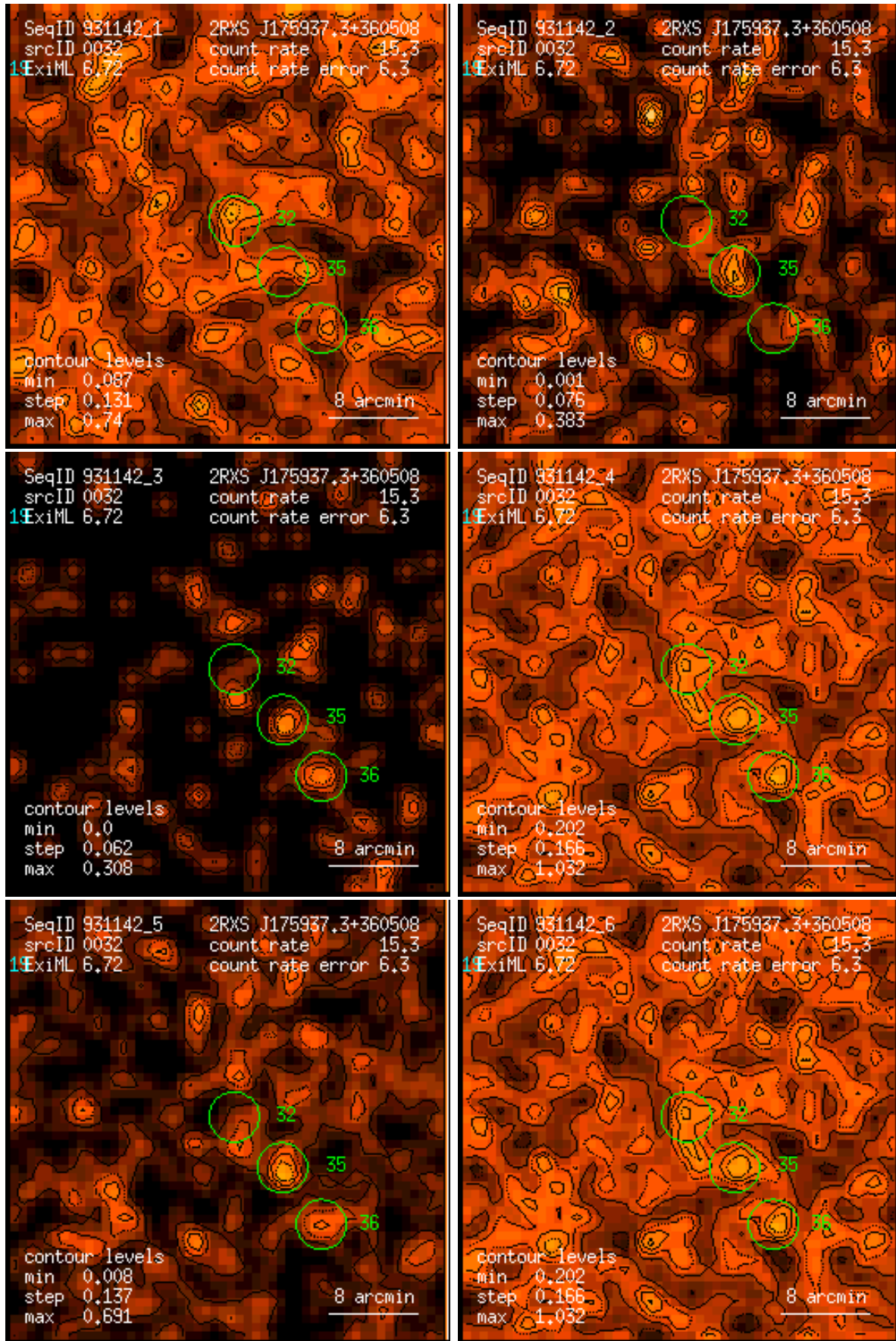
Figure 32: RASS 931142: detection 0032: band rate images, Gaussian filter: (1) PSPC channels 11 – 41, (2) 52 – 90, (3) 91 – 201, (4) 11 – 235, (5) 52 – 201, (6) 11 – 201. Broad band rates in counts/ks. Band rate contour levels in counts/ks/arcmin 2 .
