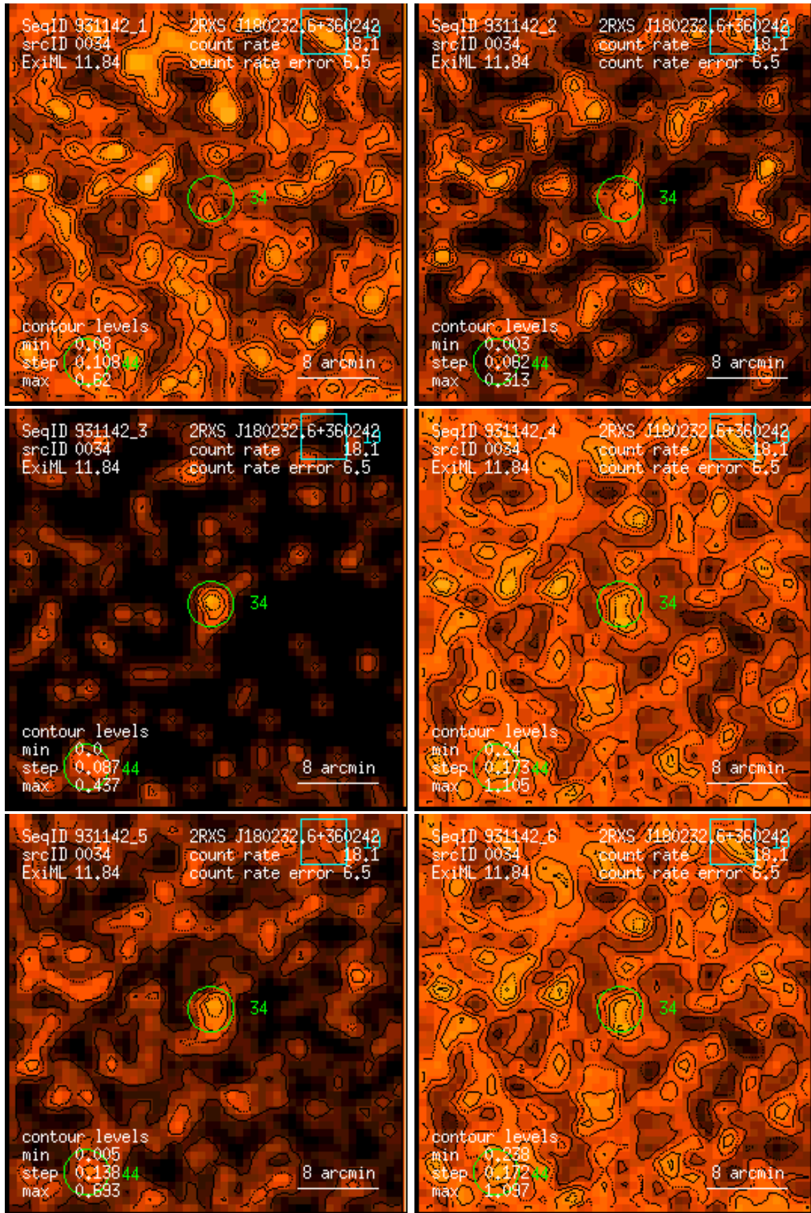
Figure 34: RASS 931142: detection 0034: band rate images, Gaussian filter: (1) PSPC channels 11 – 41, (2) 52 – 90, (3) 91 – 201, (4) 11 – 235, (5) 52 – 201, (6) 11 – 201. Broad band rates in counts/ks. Band rate contour levels in counts/ks/arcmin 2 .
