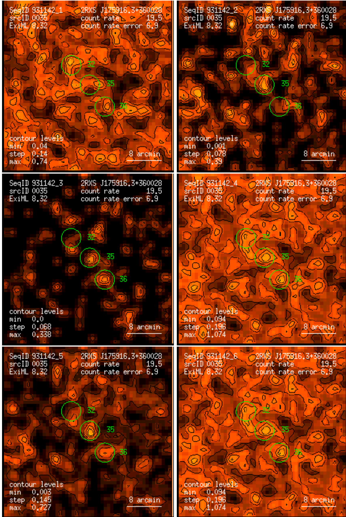
Figure 35: RASS 931142: detection 0035: band rate images, Gaussian filter: (1) PSPC channels 11 – 41, (2) 52 – 90, (3) 91 – 201, (4) 11 – 235, (5) 52 – 201, (6) 11 – 201. Broad band rates in counts/ks. Band rate contour levels in counts/ks/arcmin 2 .
