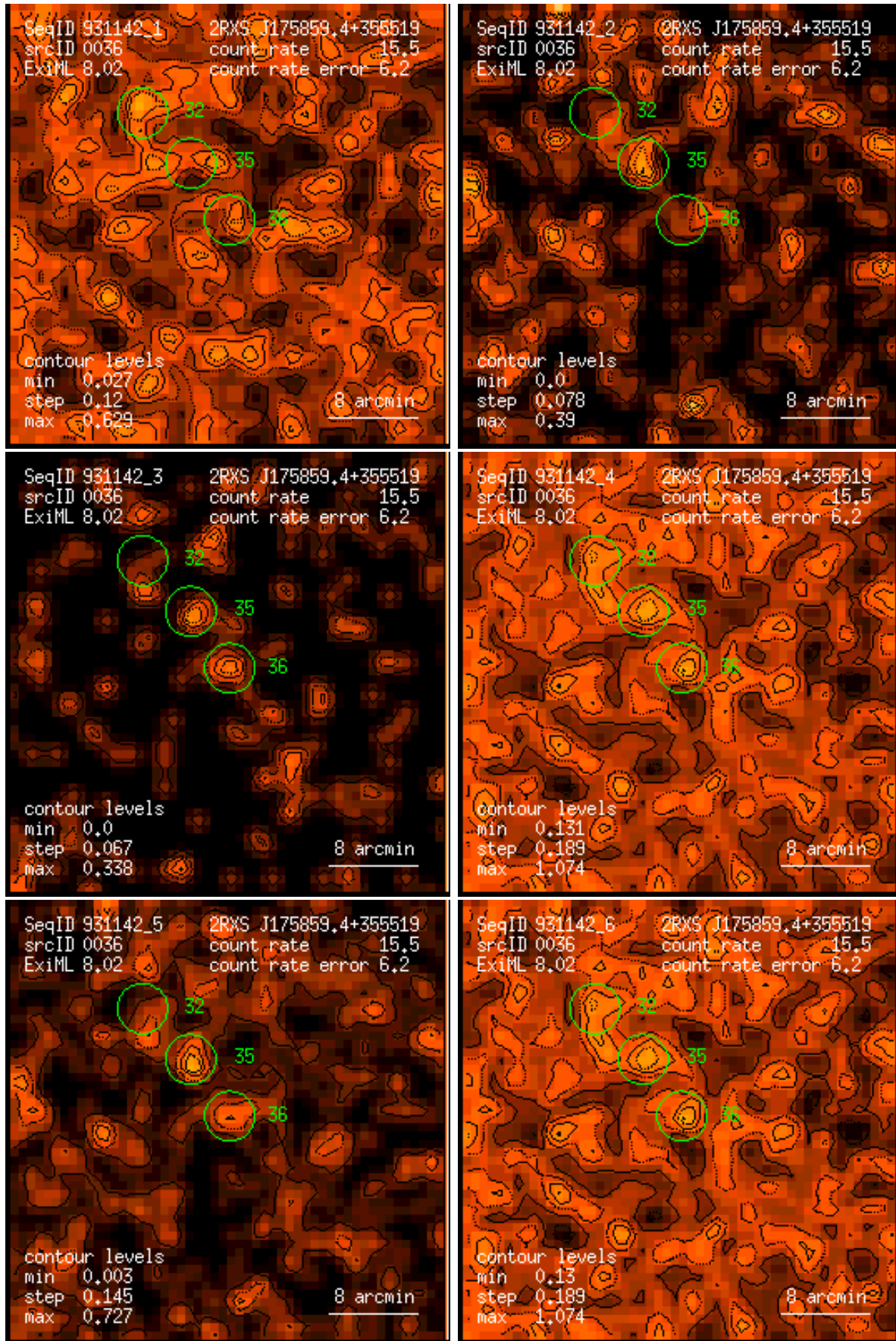
Figure 36: RASS 931142: detection 0036: band rate images, Gaussian filter: (1) PSPC channels 11 – 41, (2) 52 – 90, (3) 91 – 201, (4) 11 – 235, (5) 52 – 201, (6) 11 – 201. Broad band rates in counts/ks. Band rate contour levels in counts/ks/arcmin 2 .
