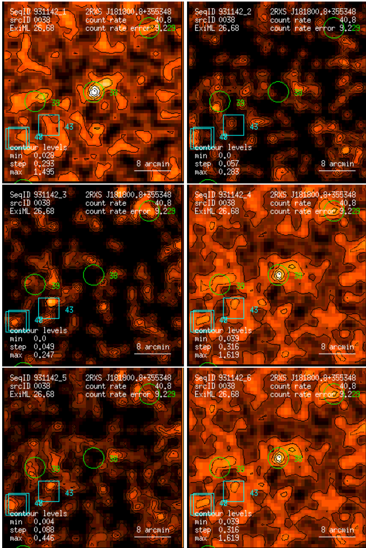
Figure 38: RASS 931142: detection 0038: band rate images, Gaussian filter: (1) PSPC channels 11 – 41, (2) 52 – 90, (3) 91 – 201, (4) 11 – 235, (5) 52 – 201, (6) 11 – 201. Broad band rates in counts/ks. Band rate contour levels in counts/ks/arcmin 2 .
