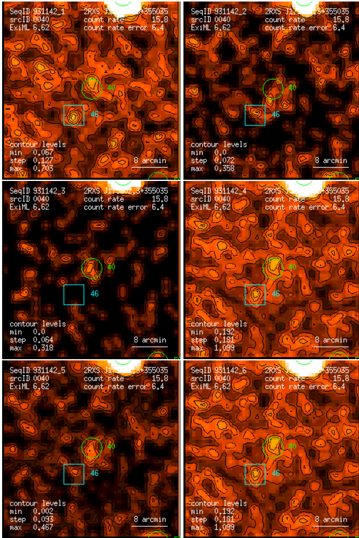
Figure 40: RASS 931142: detection 0040: band rate images, Gaussian filter: (1) PSPC channels 11 – 41, (2) 52 – 90, (3) 91 – 201, (4) 11 – 235, (5) 52 – 201, (6) 11 – 201. Broad band rates in counts/ks. Band rate contour levels in counts/ks/arcmin 2 .
