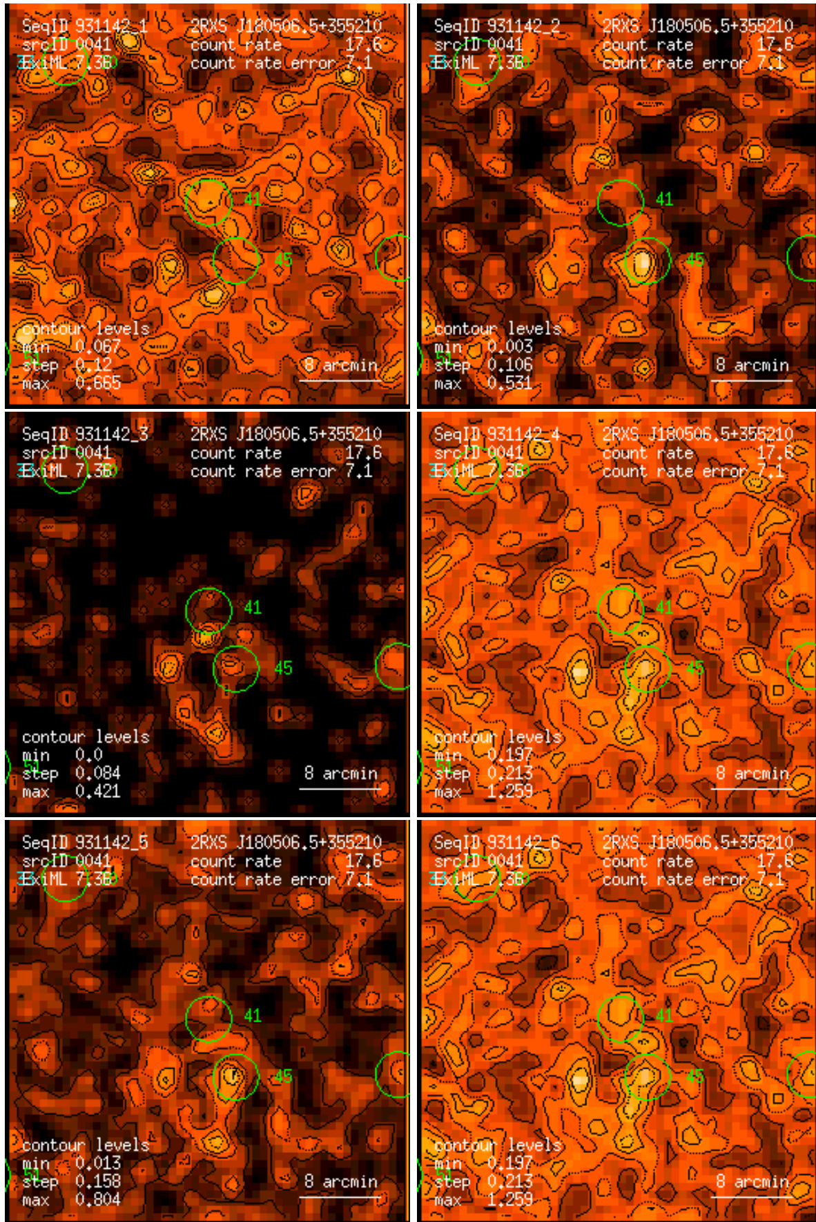
Figure 41: RASS 931142: detection 0041: band rate images, Gaussian filter: (1) PSPC channels 11 – 41, (2) 52 – 90, (3) 91 – 201, (4) 11 – 235, (5) 52 – 201, (6) 11 – 201. Broad band rates in counts/ks. Band rate contour levels in counts/ks/arcmin 2 .
