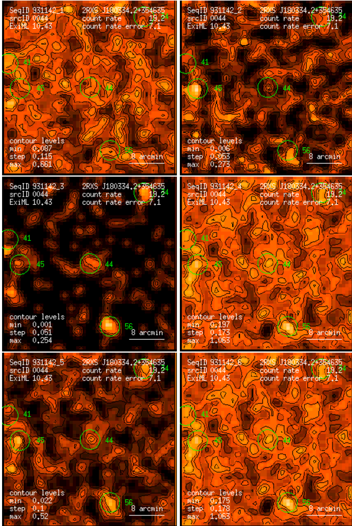
Figure 44: RASS 931142: detection 0044: band rate images, Gaussian filter: (1) PSPC channels 11 – 41, (2) 52 – 90, (3) 91 – 201, (4) 11 – 235, (5) 52 – 201, (6) 11 – 201. Broad band rates in counts/ks. Band rate contour levels in counts/ks/arcmin 2 .
