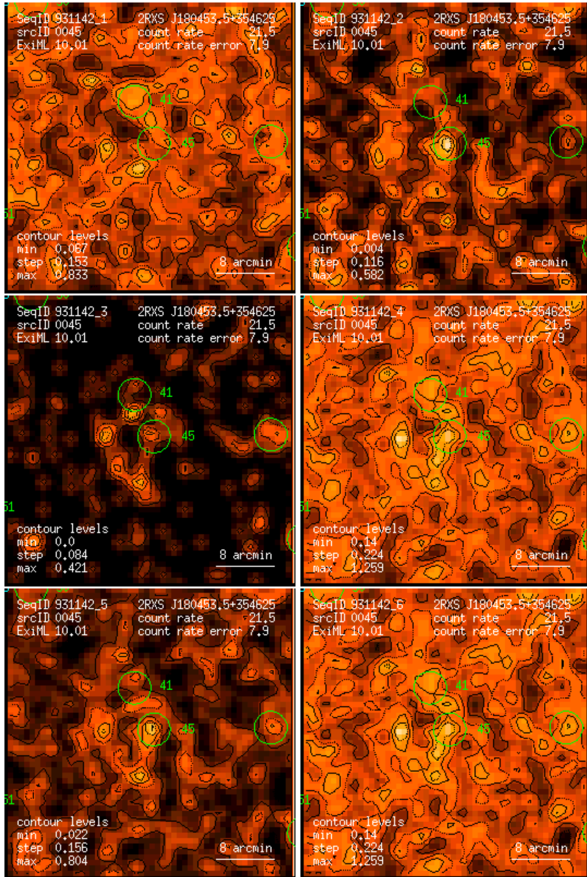
Figure 45: RASS 931142: detection 0045: band rate images, Gaussian filter: (1) PSPC channels 11 – 41, (2) 52 – 90, (3) 91 – 201, (4) 11 – 235, (5) 52 – 201, (6) 11 – 201. Broad band rates in counts/ks. Band rate contour levels in counts/ks/arcmin 2 .
