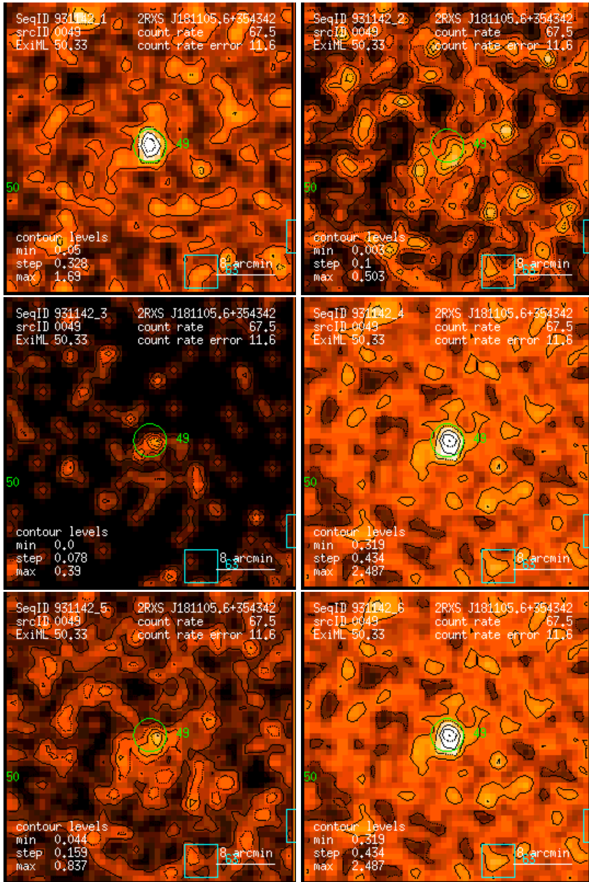
Figure 49: RASS 931142: detection 0049: band rate images, Gaussian filter: (1) PSPC channels 11 – 41, (2) 52 – 90, (3) 91 – 201, (4) 11 – 235, (5) 52 – 201, (6) 11 – 201. Broad band rates in counts/ks. Band rate contour levels in counts/ks/arcmin 2 .
