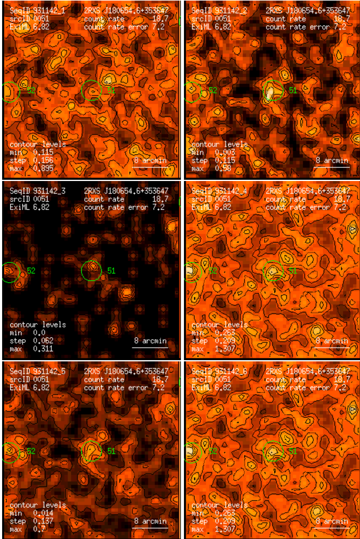
Figure 51: RASS 931142: detection 0051: band rate images, Gaussian filter: (1) PSPC channels 11 – 41, (2) 52 – 90, (3) 91 – 201, (4) 11 – 235, (5) 52 – 201, (6) 11 – 201. Broad band rates in counts/ks. Band rate contour levels in counts/ks/arcmin 2 .
