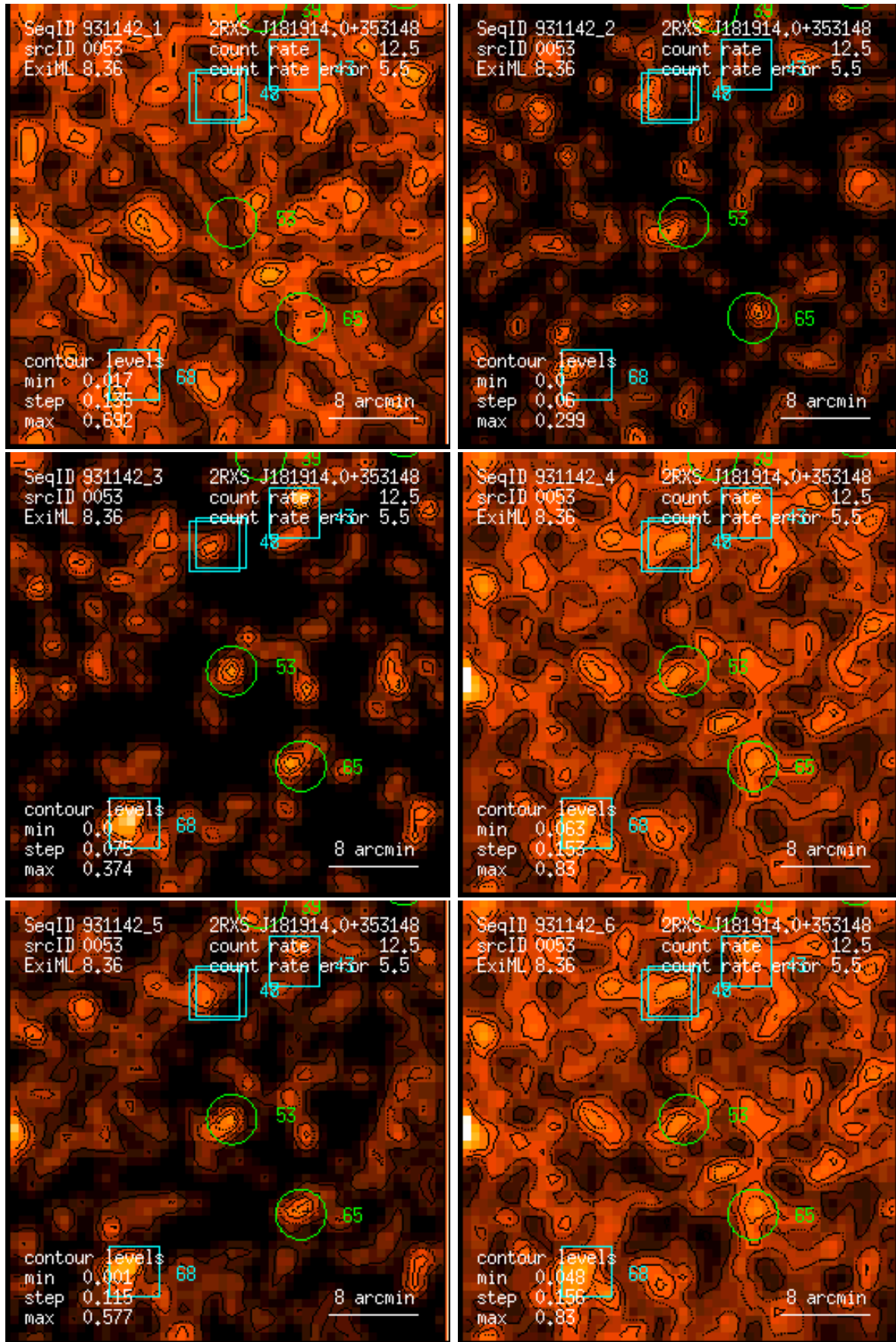
Figure 53: RASS 931142: detection 0053: band rate images, Gaussian filter: (1) PSPC channels 11 – 41, (2) 52 – 90, (3) 91 – 201, (4) 11 – 235, (5) 52 – 201, (6) 11 – 201. Broad band rates in counts/ks. Band rate contour levels in counts/ks/arcmin 2 .
