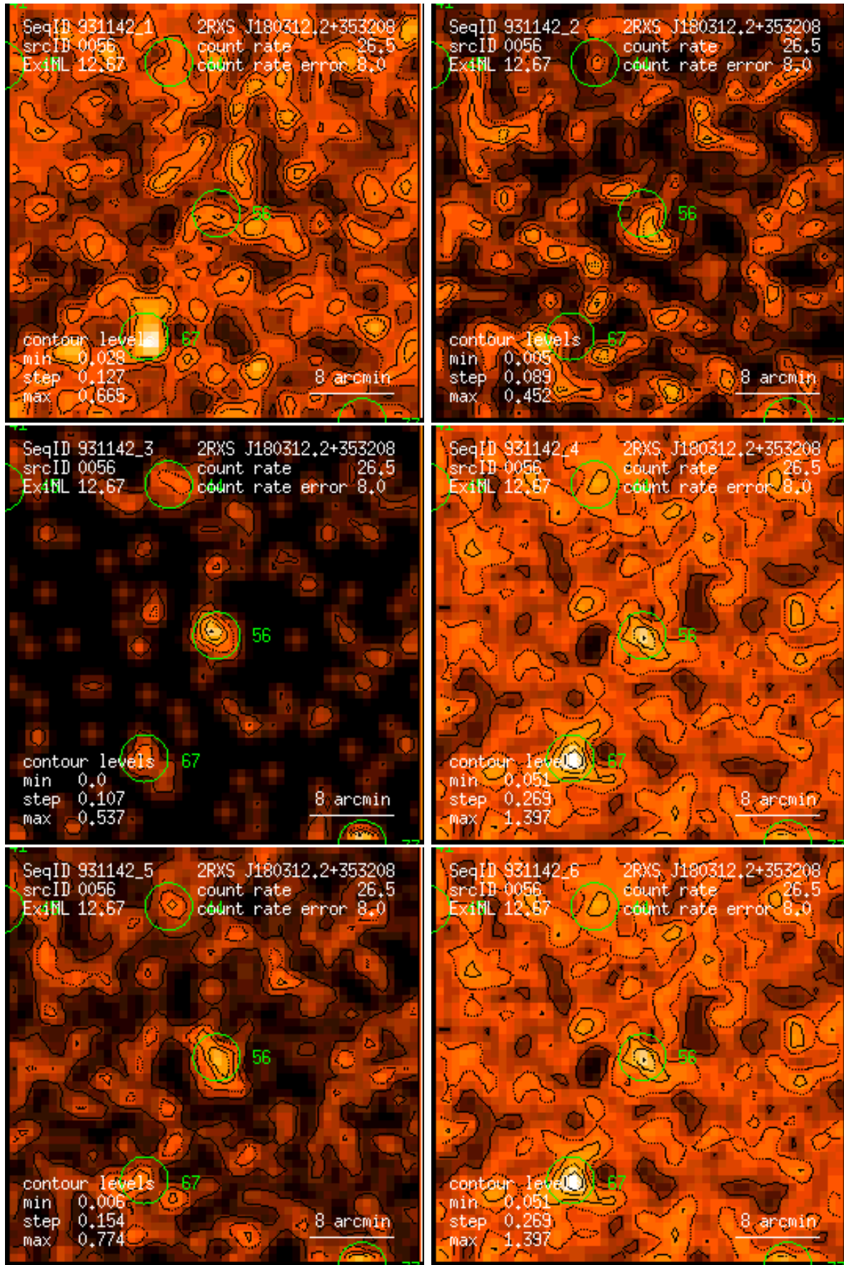
Figure 56: RASS 931142: detection 0056: band rate images, Gaussian filter: (1) PSPC channels 11 – 41, (2) 52 – 90, (3) 91 – 201, (4) 11 – 235, (5) 52 – 201, (6) 11 – 201. Broad band rates in counts/ks. Band rate contour levels in counts/ks/arcmin 2 .
