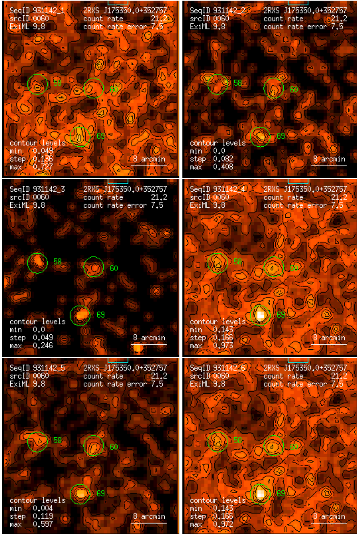
Figure 60: RASS 931142: detection 0060: band rate images, Gaussian filter: (1) PSPC channels 11 – 41, (2) 52 – 90, (3) 91 – 201, (4) 11 – 235, (5) 52 – 201, (6) 11 – 201. Broad band rates in counts/ks. Band rate contour levels in counts/ks/arcmin 2 .
