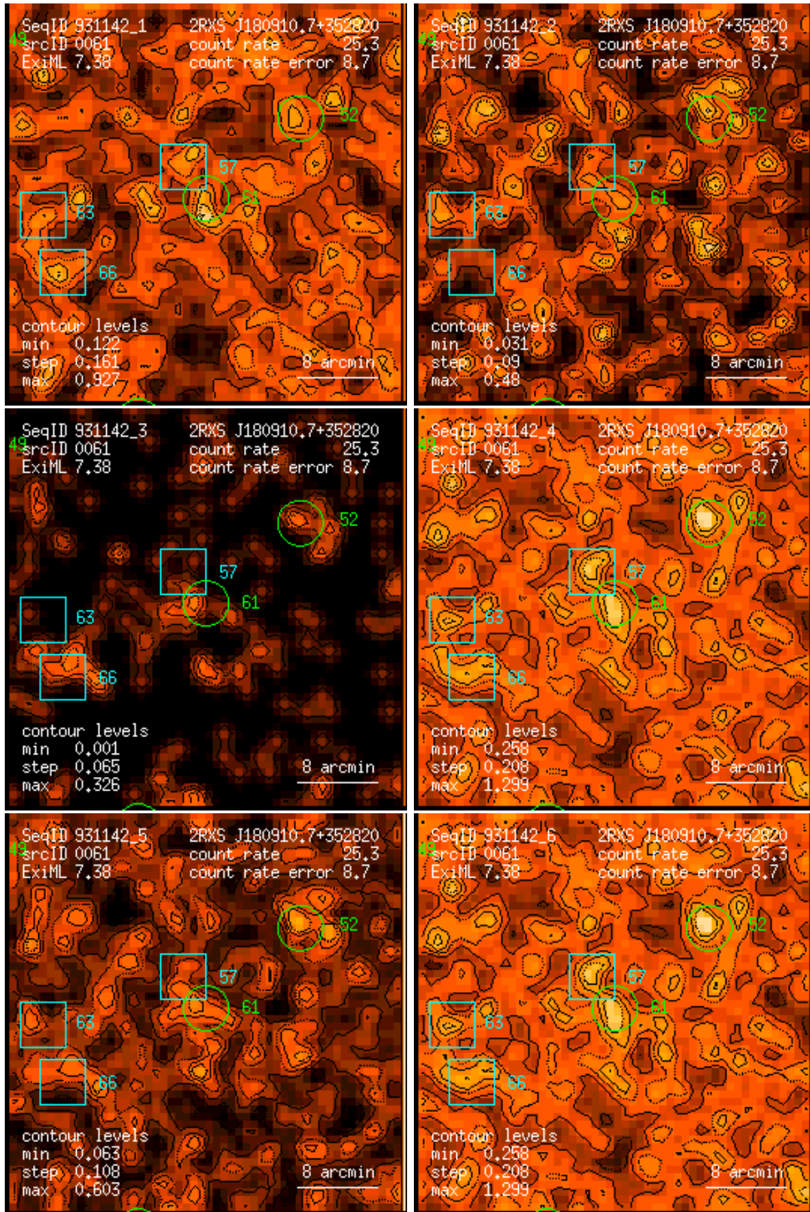
Figure 61: RASS 931142: detection 0061: band rate images, Gaussian filter: (1) PSPC channels 11 – 41, (2) 52 – 90, (3) 91 – 201, (4) 11 – 235, (5) 52 – 201, (6) 11 – 201. Broad band rates in counts/ks. Band rate contour levels in counts/ks/arcmin 2 .
