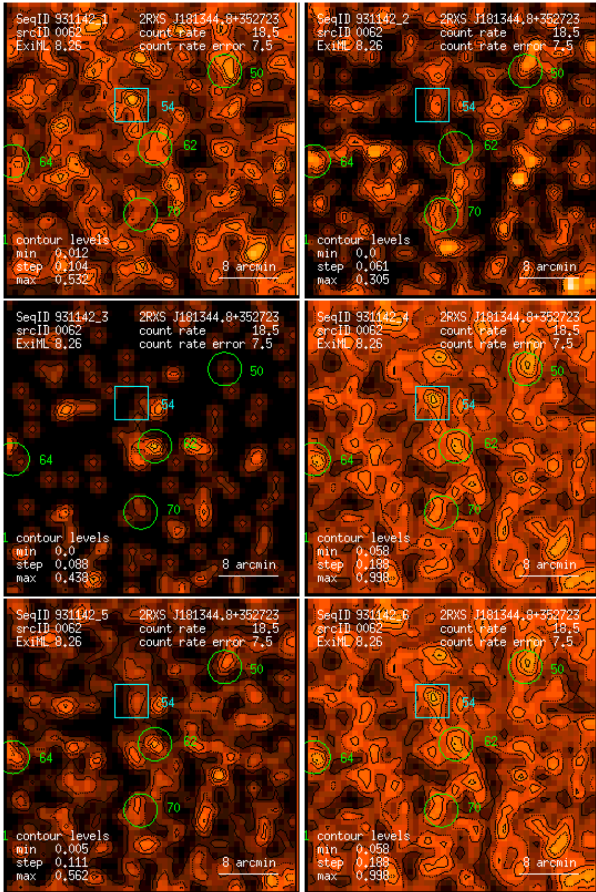
Figure 62: RASS 931142: detection 0062: band rate images, Gaussian filter: (1) PSPC channels 11 – 41, (2) 52 – 90, (3) 91 – 201, (4) 11 – 235, (5) 52 – 201, (6) 11 – 201. Broad band rates in counts/ks. Band rate contour levels in counts/ks/arcmin 2 .
