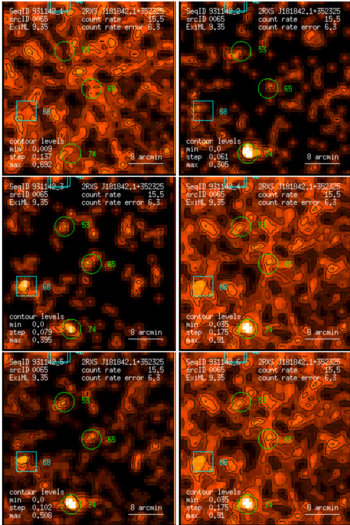
Figure 65: RASS 931142: detection 0065: band rate images, Gaussian filter: (1) PSPC channels 11 – 41, (2) 52 – 90, (3) 91 – 201, (4) 11 – 235, (5) 52 – 201, (6) 11 – 201. Broad band rates in counts/ks. Band rate contour levels in counts/ks/arcmin 2 .
