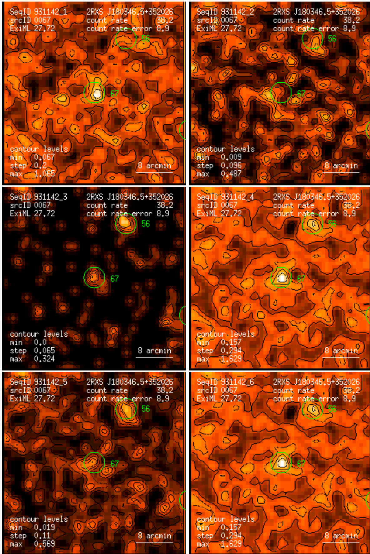
Figure 67: RASS 931142: detection 0067: band rate images, Gaussian filter: (1) PSPC channels 11 – 41, (2) 52 – 90, (3) 91 – 201, (4) 11 – 235, (5) 52 – 201, (6) 11 – 201. Broad band rates in counts/ks. Band rate contour levels in counts/ks/arcmin 2 .
