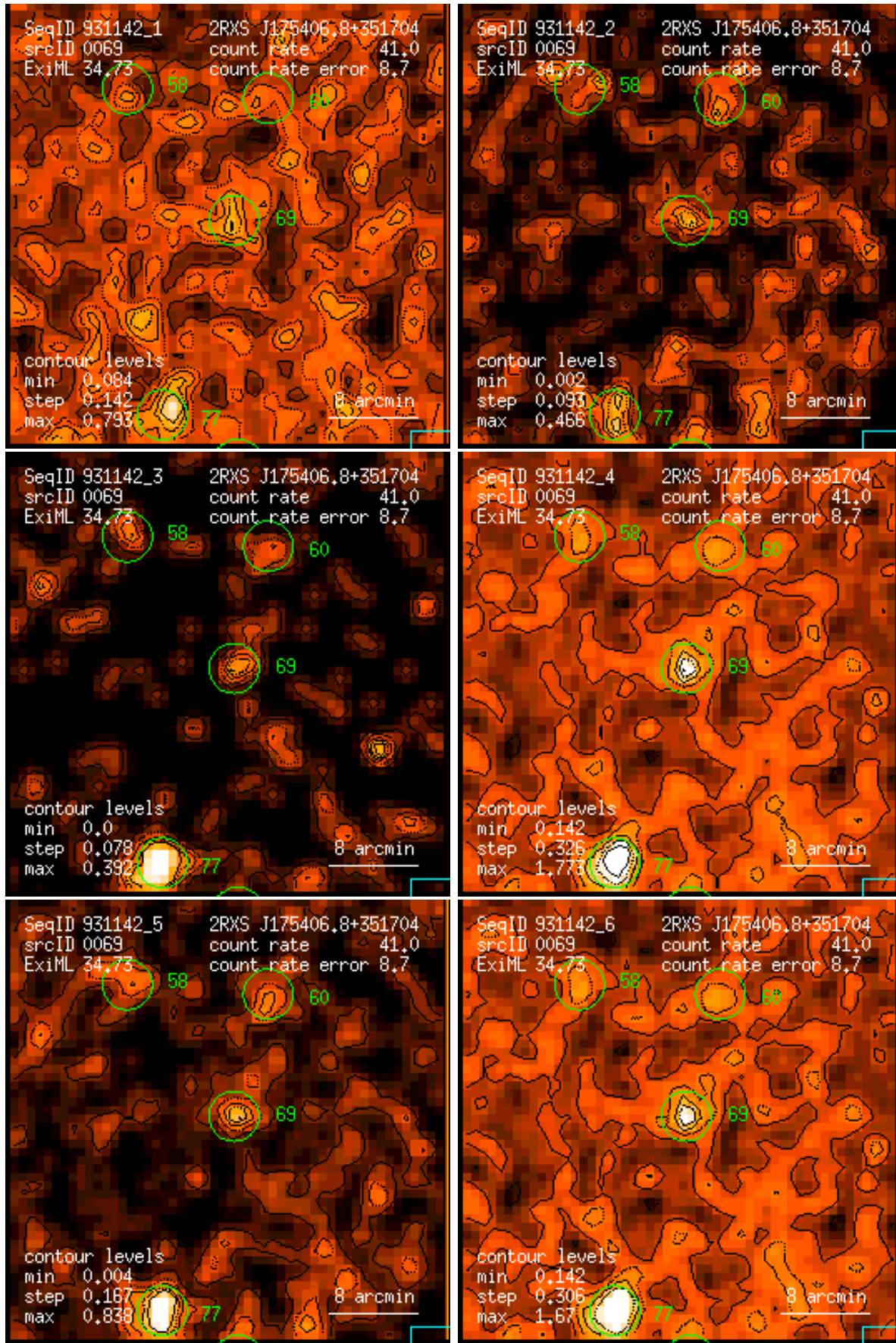
Figure 69: RASS 931142: detection 0069: band rate images, Gaussian filter: (1) PSPC channels 11 – 41, (2) 52 – 90, (3) 91 – 201, (4) 11 – 235, (5) 52 – 201, (6) 11 – 201. Broad band rates in counts/ks. Band rate contour levels in counts/ks/arcmin 2 .
